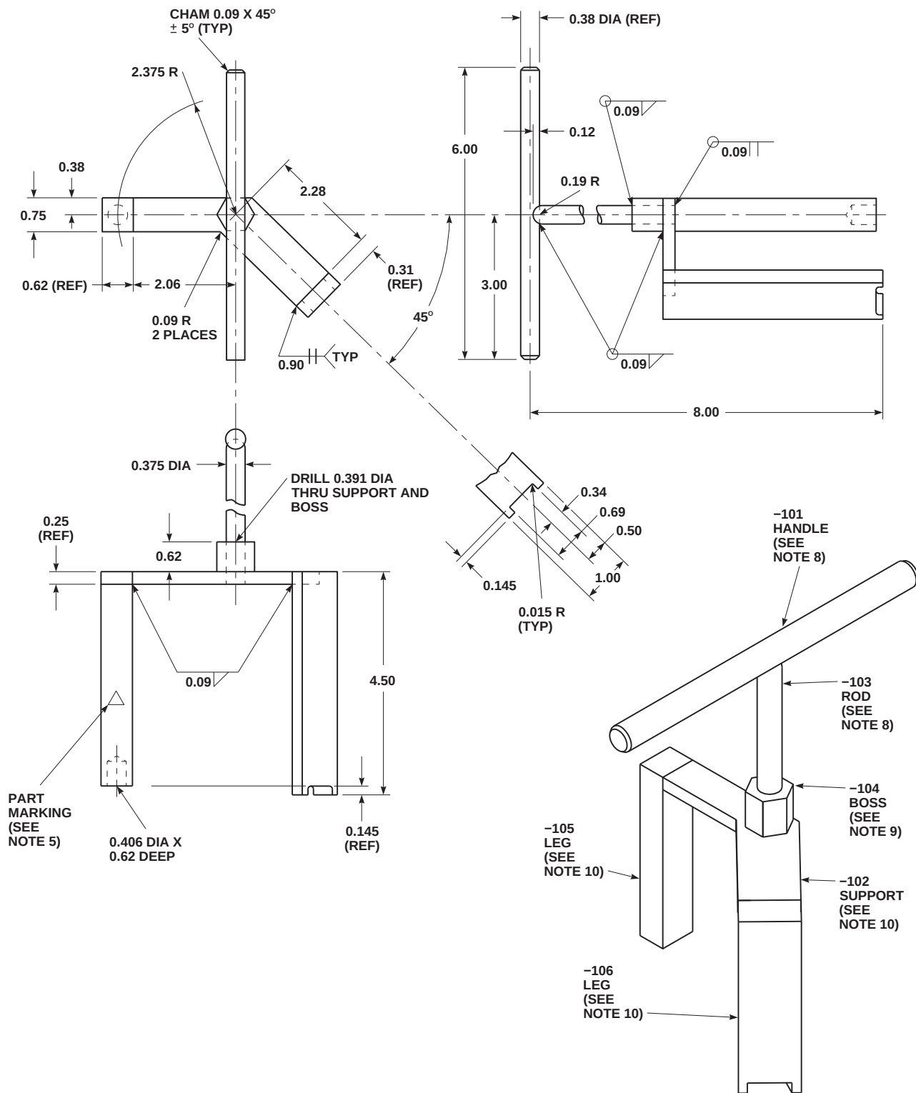
POSITIONER TOOL
