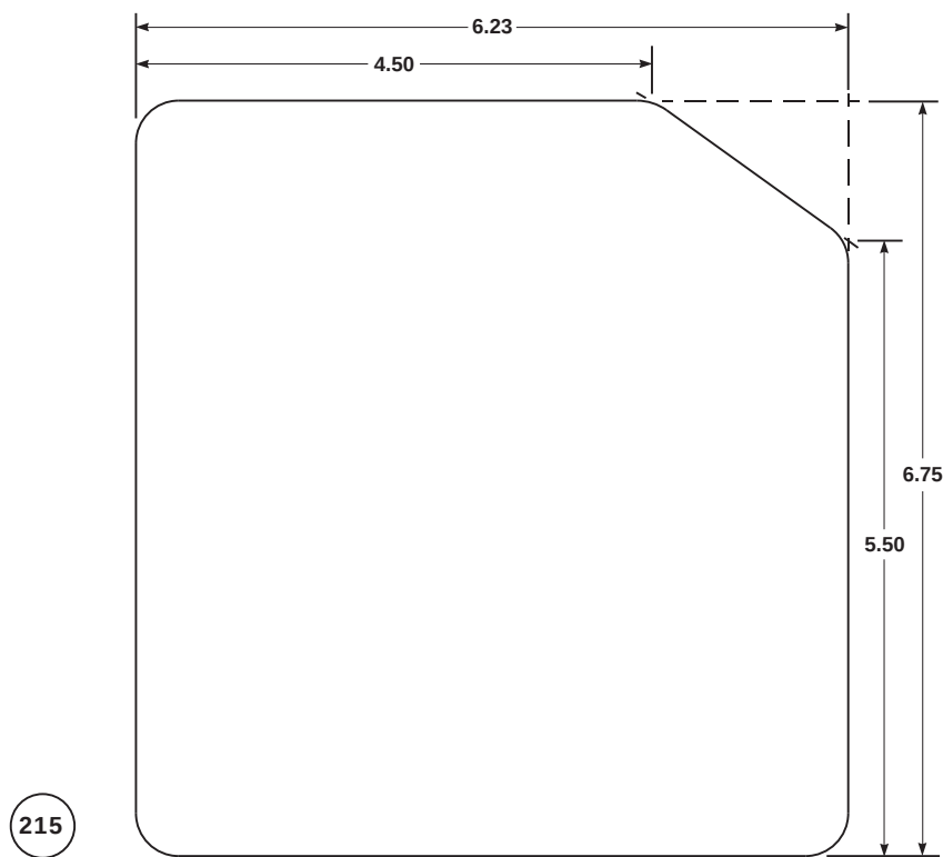
FIGURE H-131. FOIL PANEL UNUSUAL CONFIGURATION (SHEET 16 OF 43)
