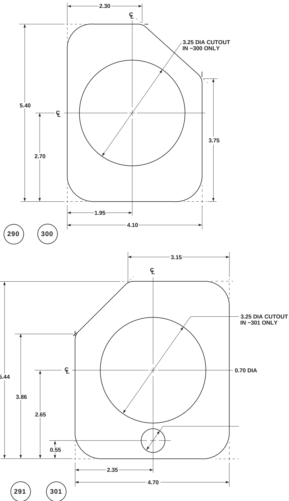
FIGURE H-131. FOIL PANEL UNUSUAL CONFIGURATION (SHEET 34 OF 43)
