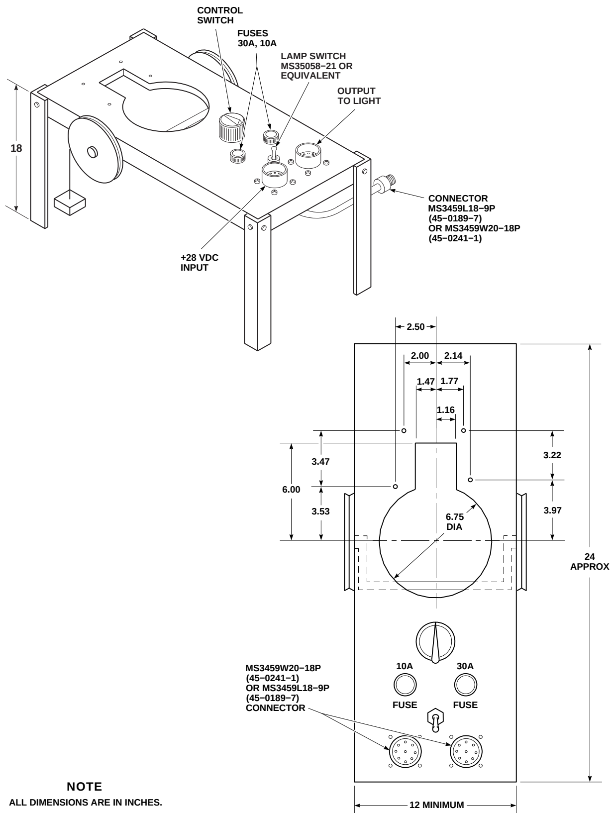
FIGURE H-249 SEARCHLIGHT TEST STAND (SHEET 1 OF 4)
