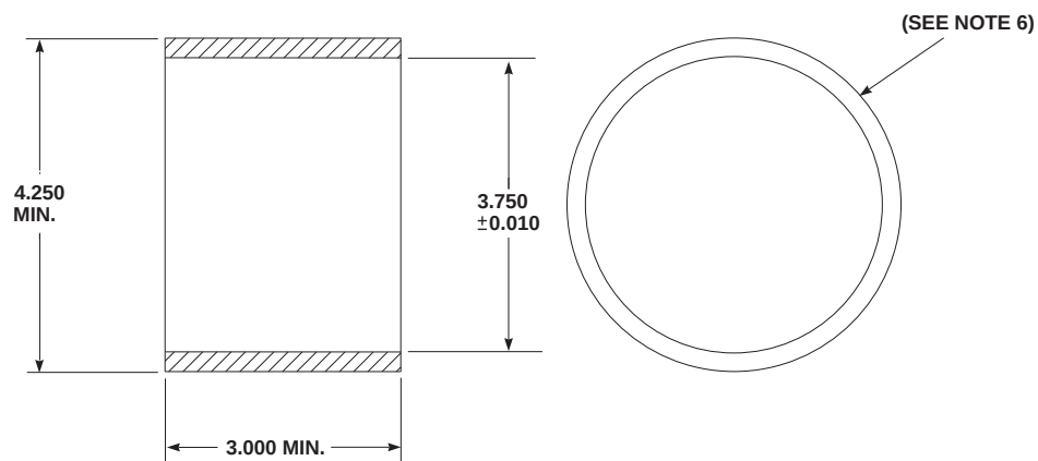
SPHERICAL BEARING SUPPORT (REMOVAL) P/N AV15-1992
