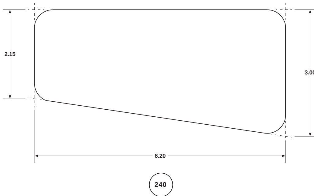
FIGURE H-131. FOIL PANEL UNUSUAL CONFIGURATION (SHEET 19 OF 43)
