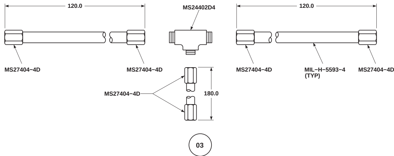
TEE AIR HOSE ASSEMBLY (AFCS)
