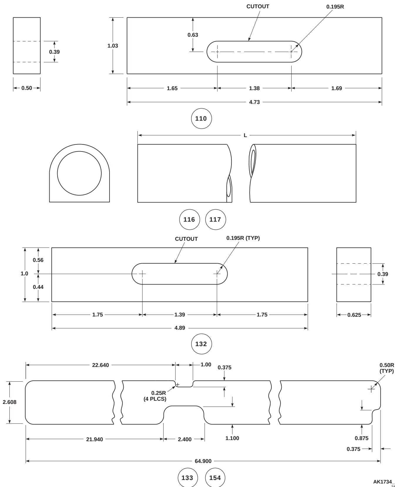
FIGURE H-76. CABIN DOOR SEAL (SHEET 1 OF 3)
