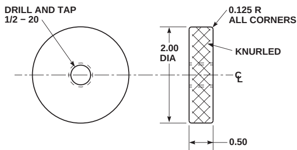
DETAIL C HANDWHEEL
