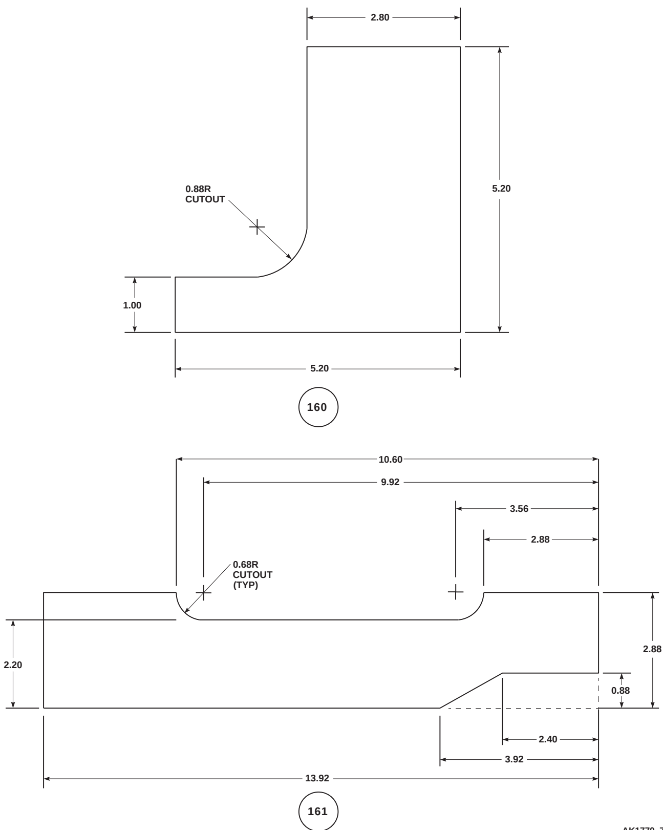
FIGURE H-131. FOIL PANEL UNUSUAL CONFIGURATION (SHEET 7 OF 43)
