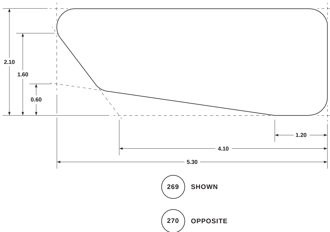
FIGURE H-131. FOIL PANEL UNUSUAL CONFIGURATION (SHEET 28 OF 43)
