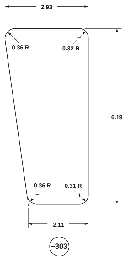
FIGURE H-131. FOIL PANEL UNUSUAL CONFIGURATION (SHEET 37 OF 43)
