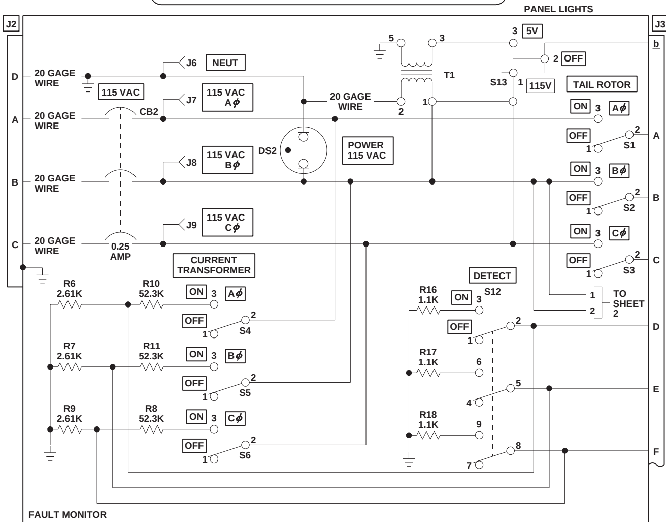
FIGURE H-155. BLADE DEICE TEST SET (SHEET 1 OF 4)
