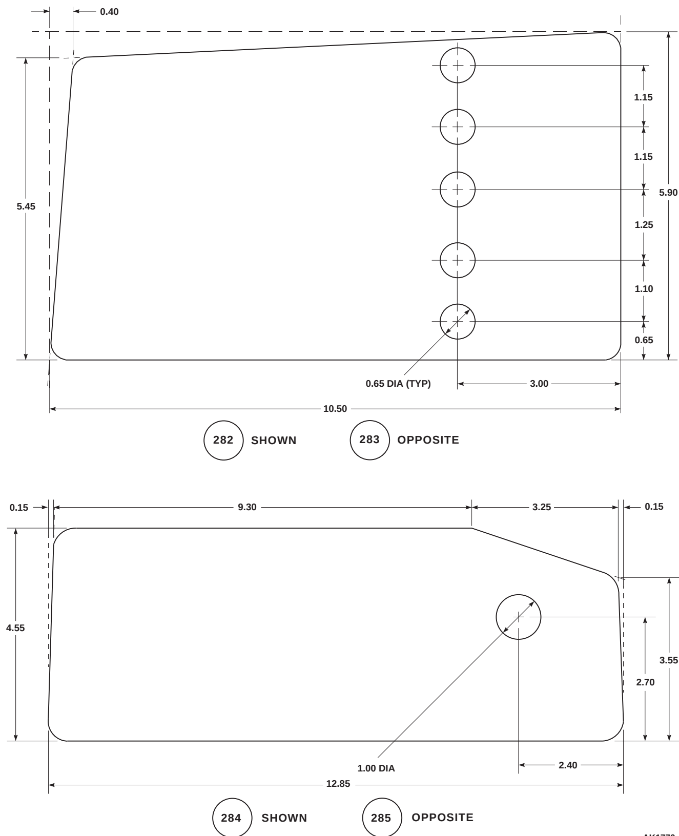
FIGURE H-131. FOIL PANEL UNUSUAL CONFIGURATION (SHEET 31 OF 43)
