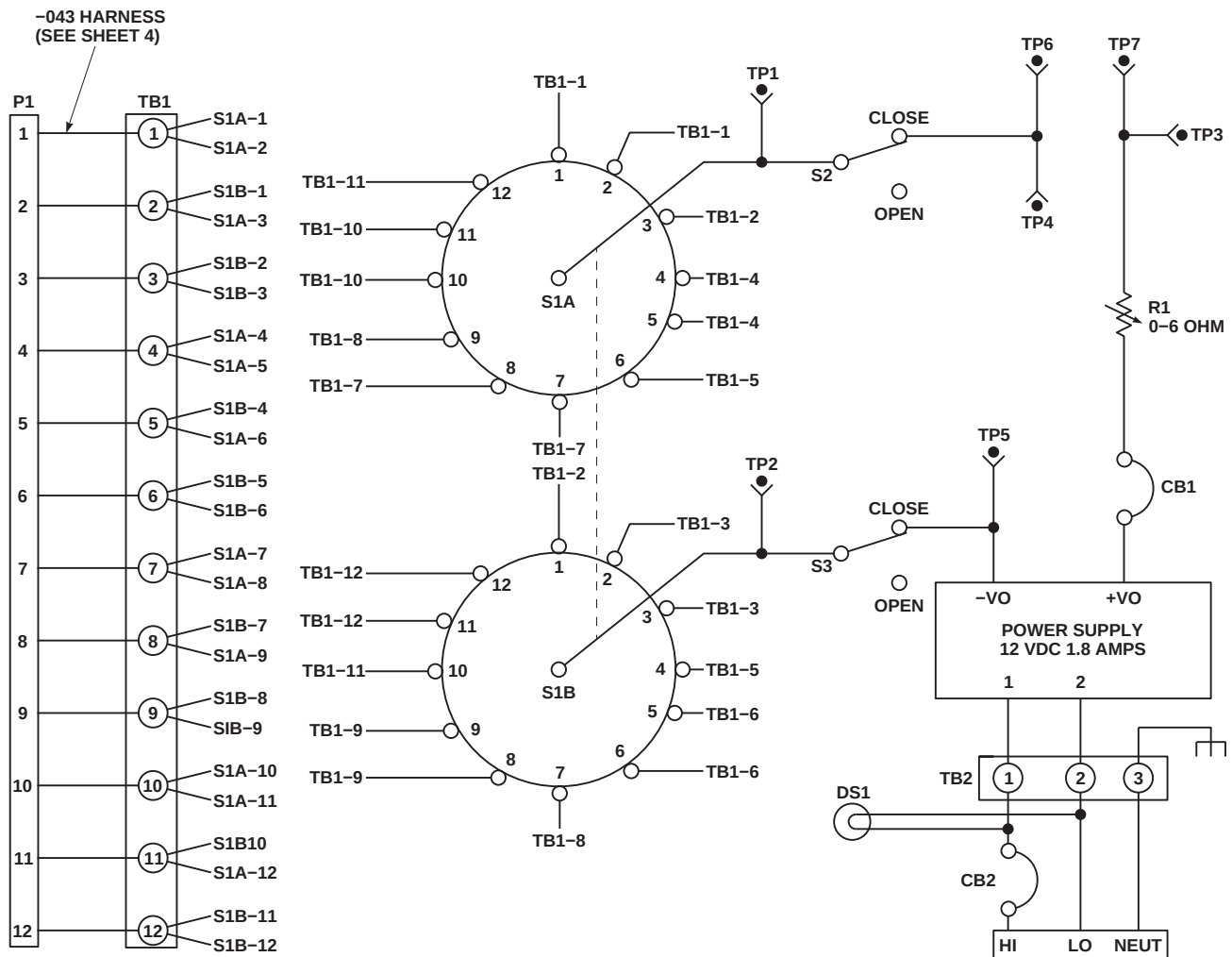
HEATER MAT RESISTANCE TEST SET
