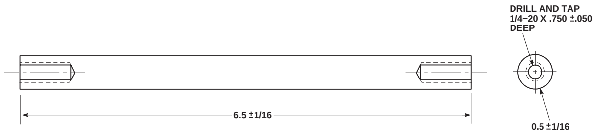
DETAIL C
