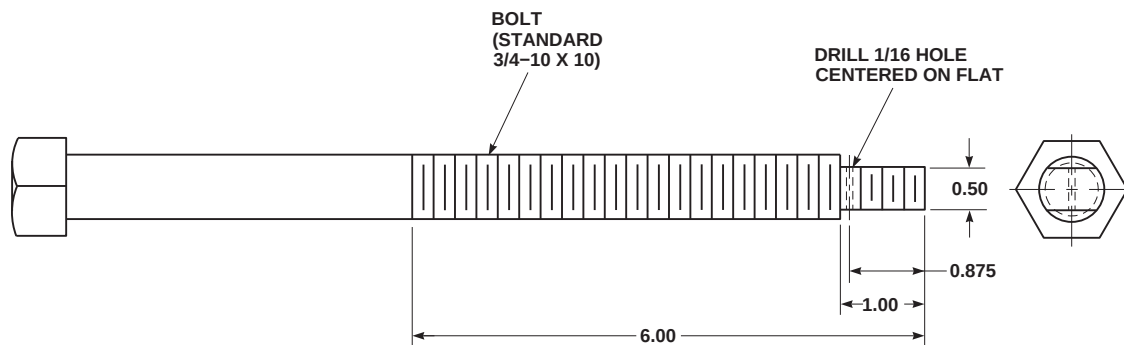
DETAIL D
