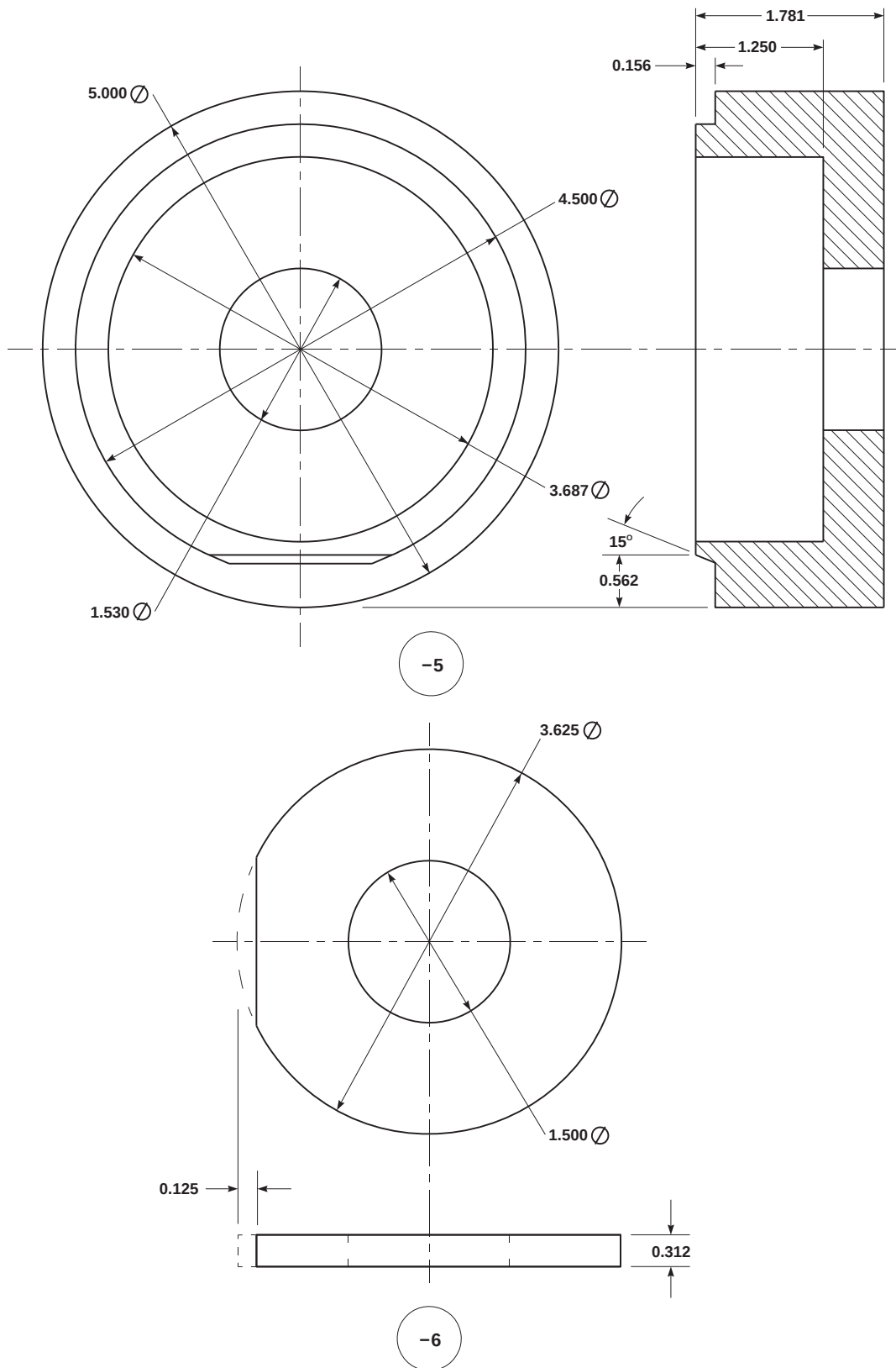
FIGURE H-213. BIFILAR BUSHINGS REPLACEMENT TOOLS (SHEET 3 OF 5)
