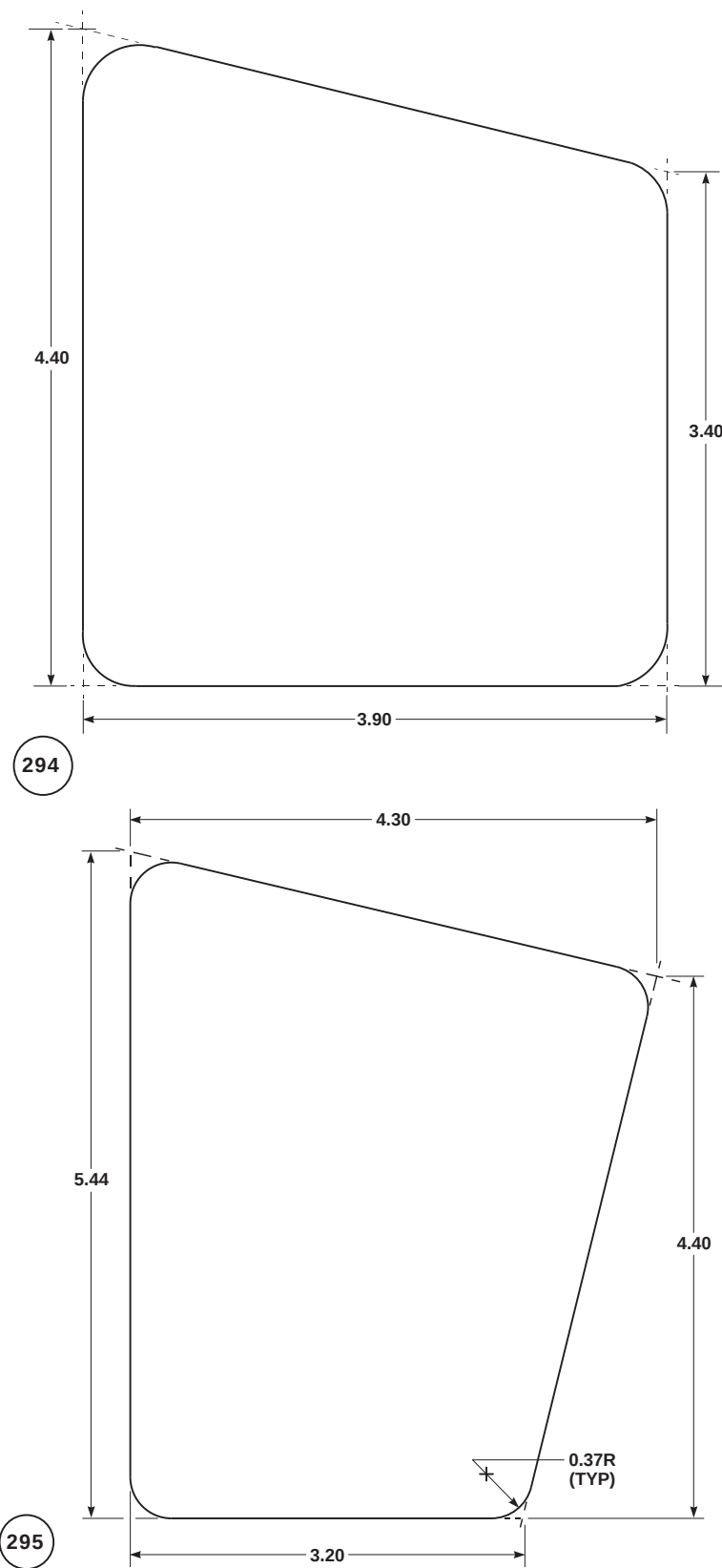
FIGURE H-131. FOIL PANEL UNUSUAL CONFIGURATION (SHEET 36 OF 43)
