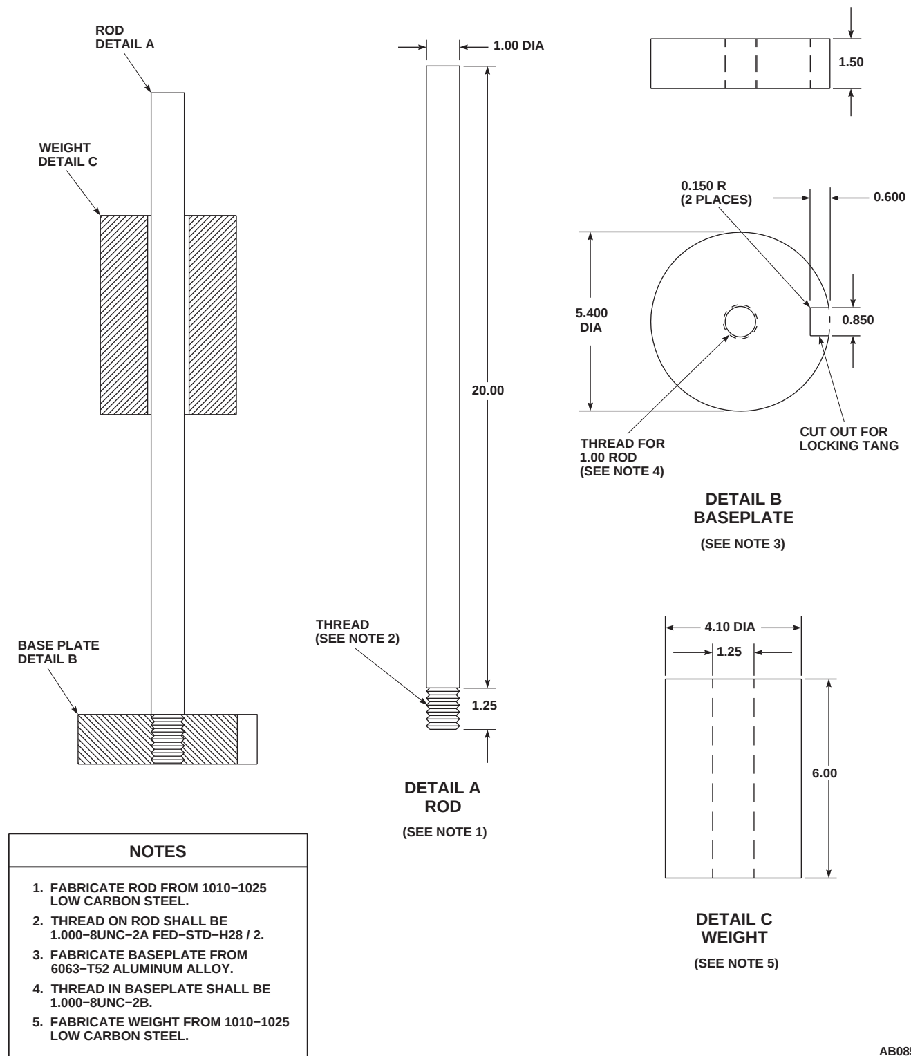
FIGURE H-252. MAIN ROTOR SHAFT IMPACT TOOL
