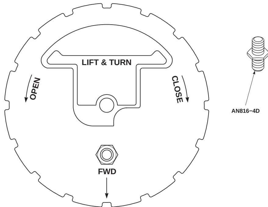
FIGURE H-212. FUEL CELL CAP PRESSURE TEST ADAPTER
