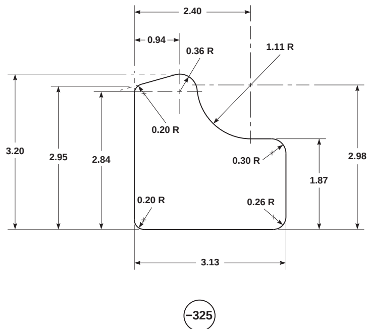
FIGURE H-131. FOIL PANEL UNUSUAL CONFIGURATION (SHEET 41 OF 43)
