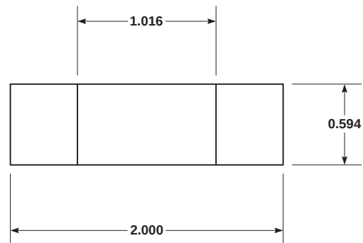
FIGURE H-267. ORIFICE ASSEMBLY GAGE
