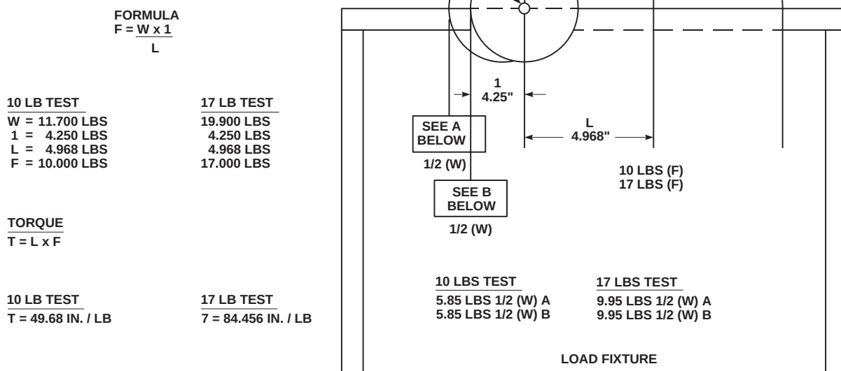
FIGURE H-249. SEARCHLIGHT TEST STAND (SHEET 2 OF 4)
