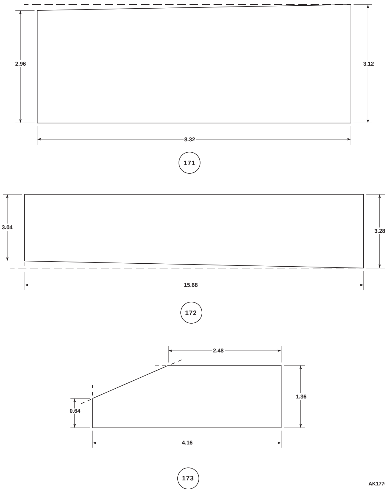
FIGURE H-131. FOIL PANEL UNUSUAL CONFIGURATION (SHEET 9 OF 43)
