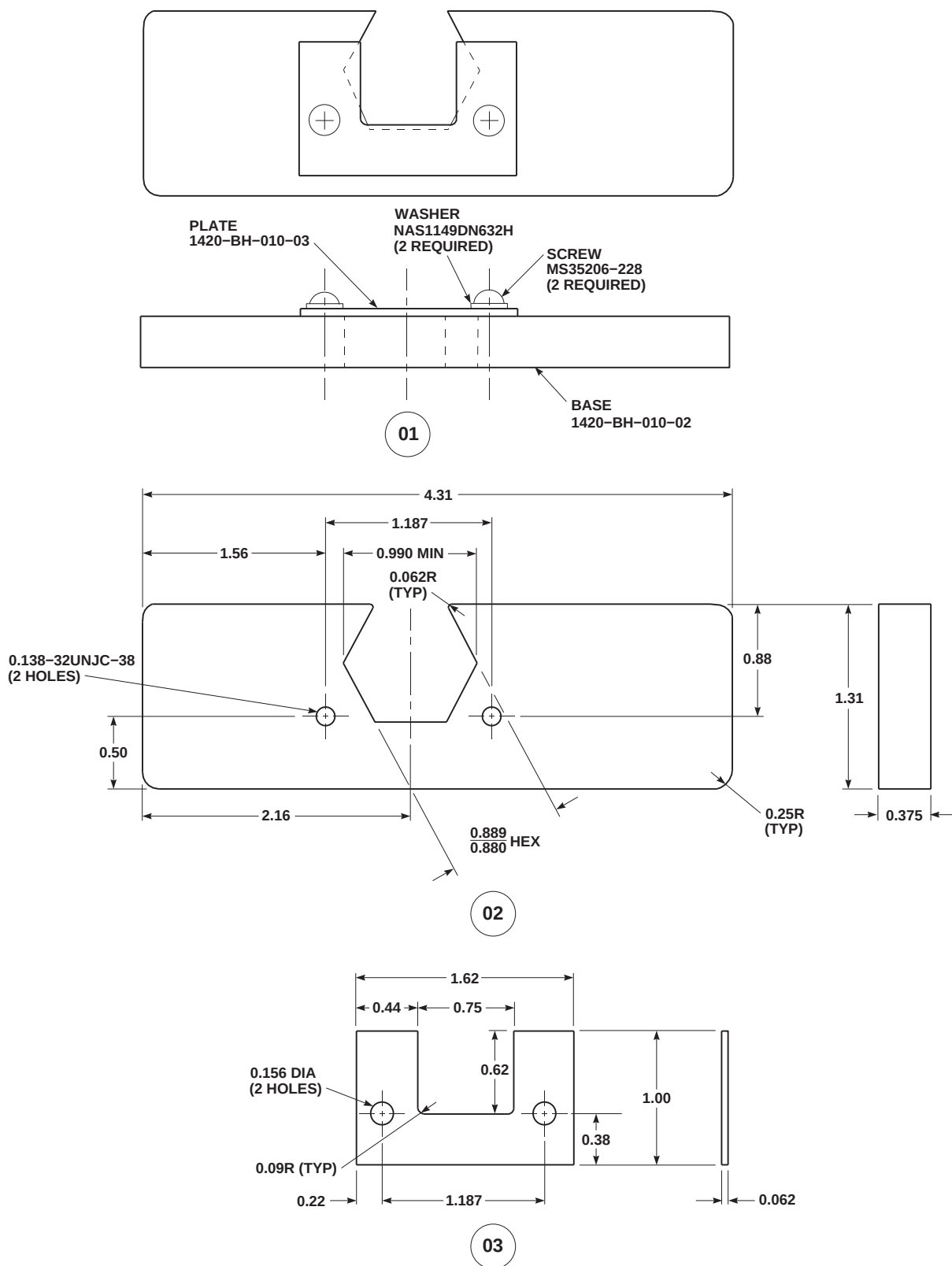
FIGURE H-48. FLIGHT CONTROL QUICK-DISCONNECT WRENCH (SHEET 1 OF 2)
