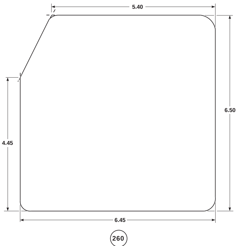
FIGURE H-131. FOIL PANEL UNUSUAL CONFIGURATION (SHEET 26 OF 43)
