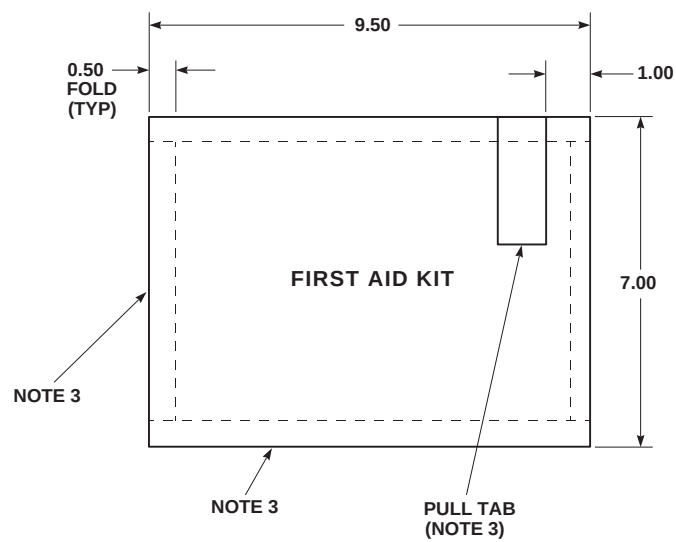
COVER FOLDED FOR SEWING
