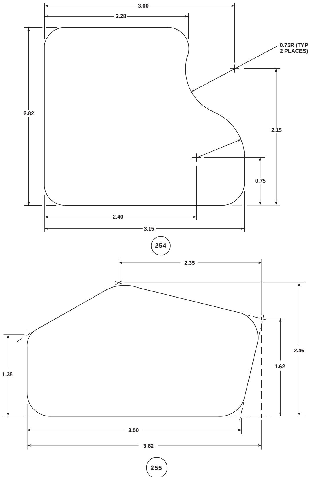
FIGURE H-131. FOIL PANEL UNUSUAL CONFIGURATION (SHEET 24 OF 43)
