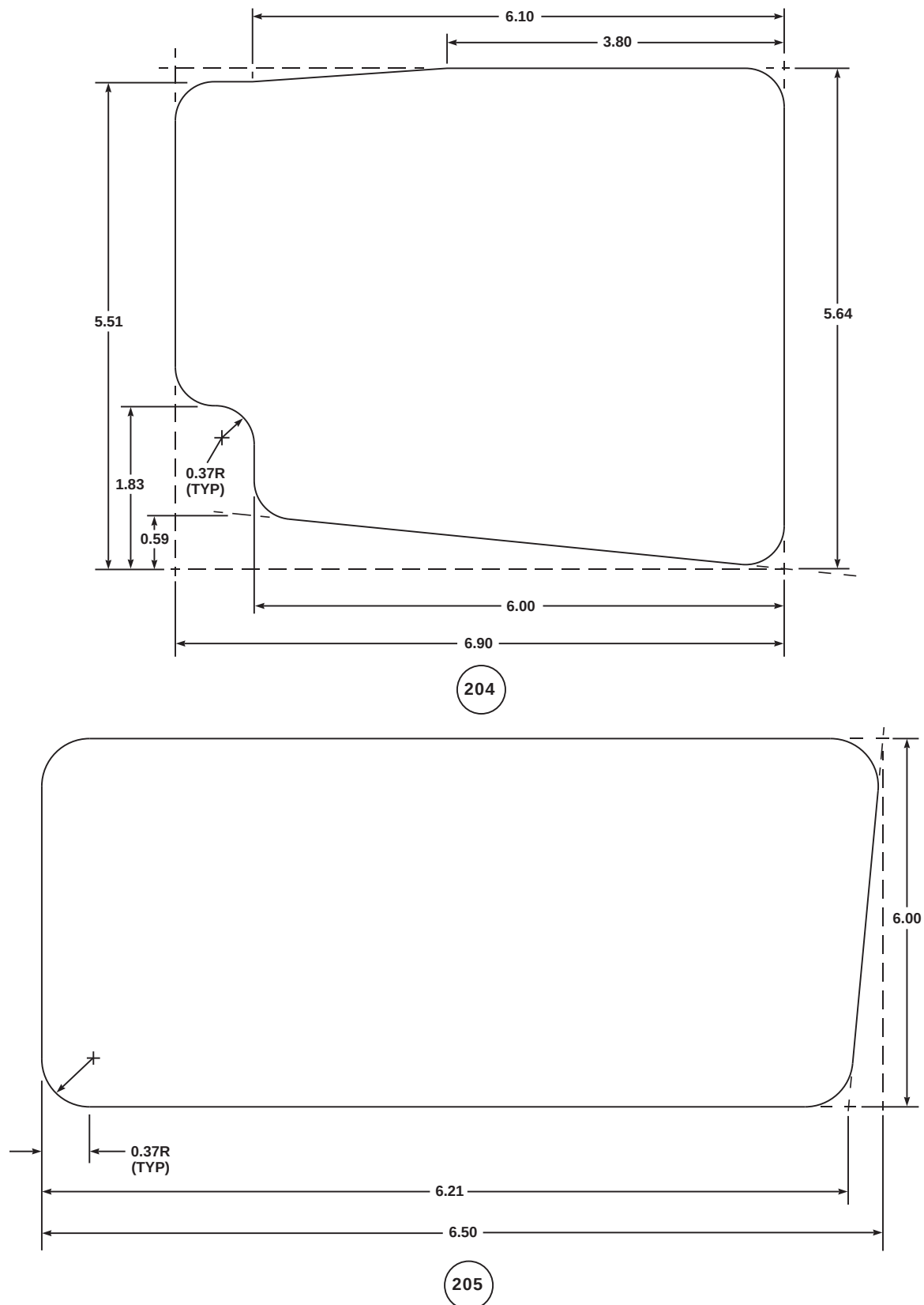
FIGURE H-131. FOIL PANEL UNUSUAL CONFIGURATION (SHEET 12 OF 43)
