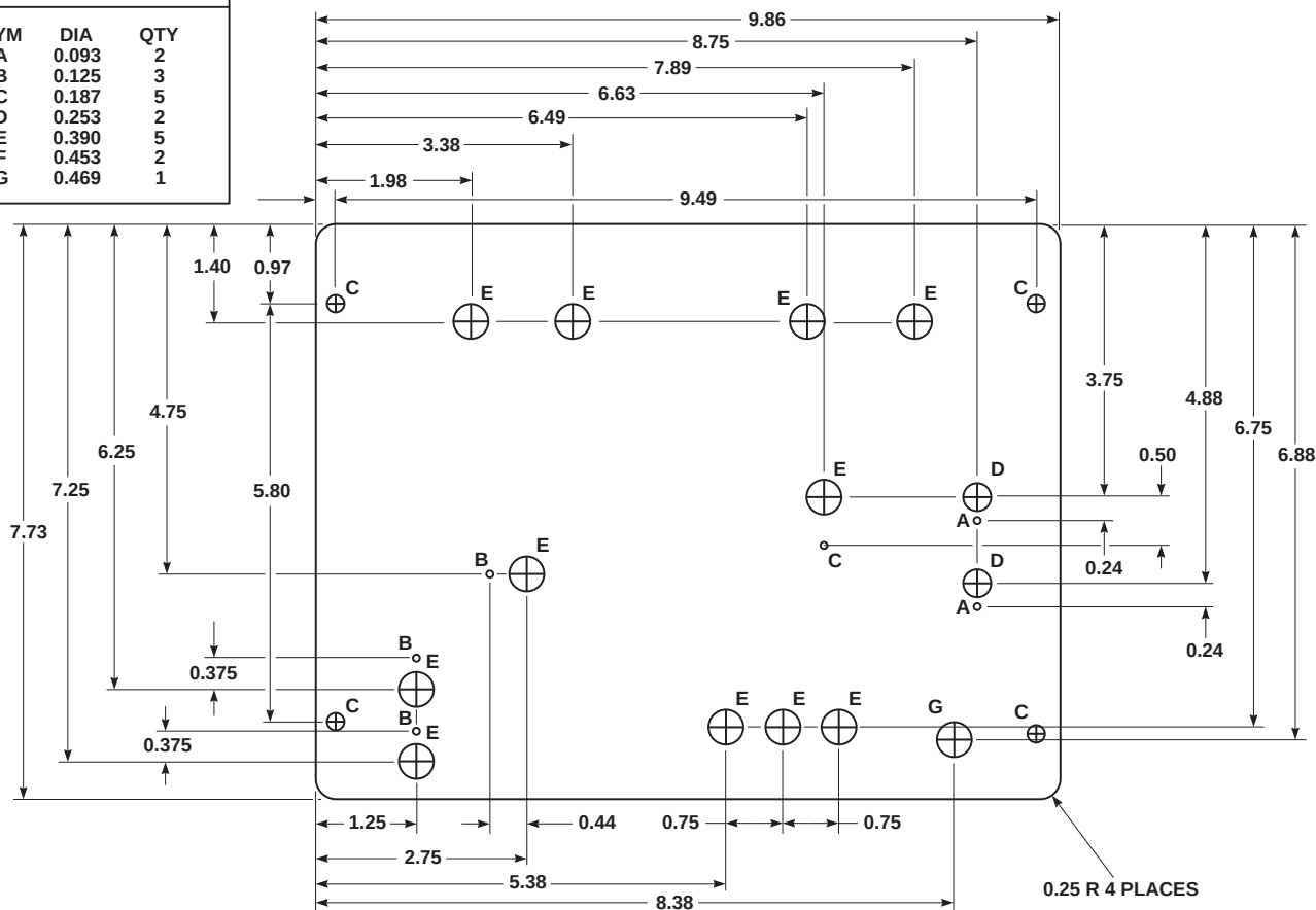
HEATER MAT RESISTANCE TEST SET FRONT PANEL LAYOUT
