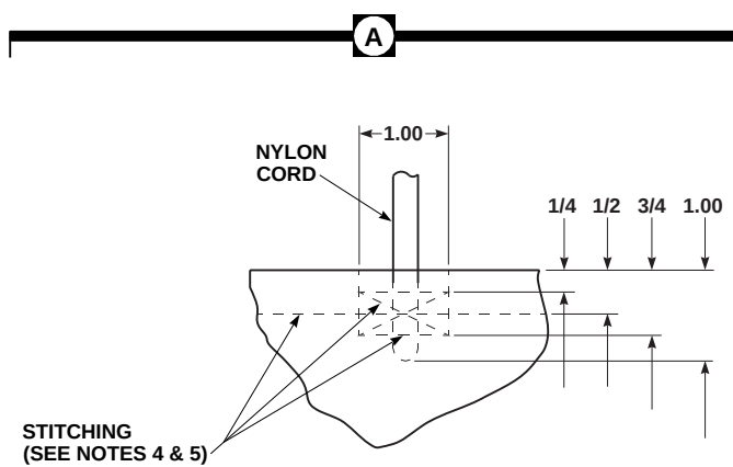
FIGURE H-192. MAST COVER (SHEET 1 OF 2)
