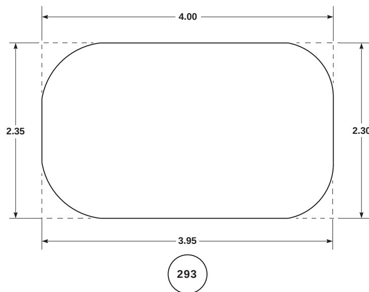
FIGURE H-131. FOIL PANEL UNUSUAL CONFIGURATION (SHEET 35 OF 43)
