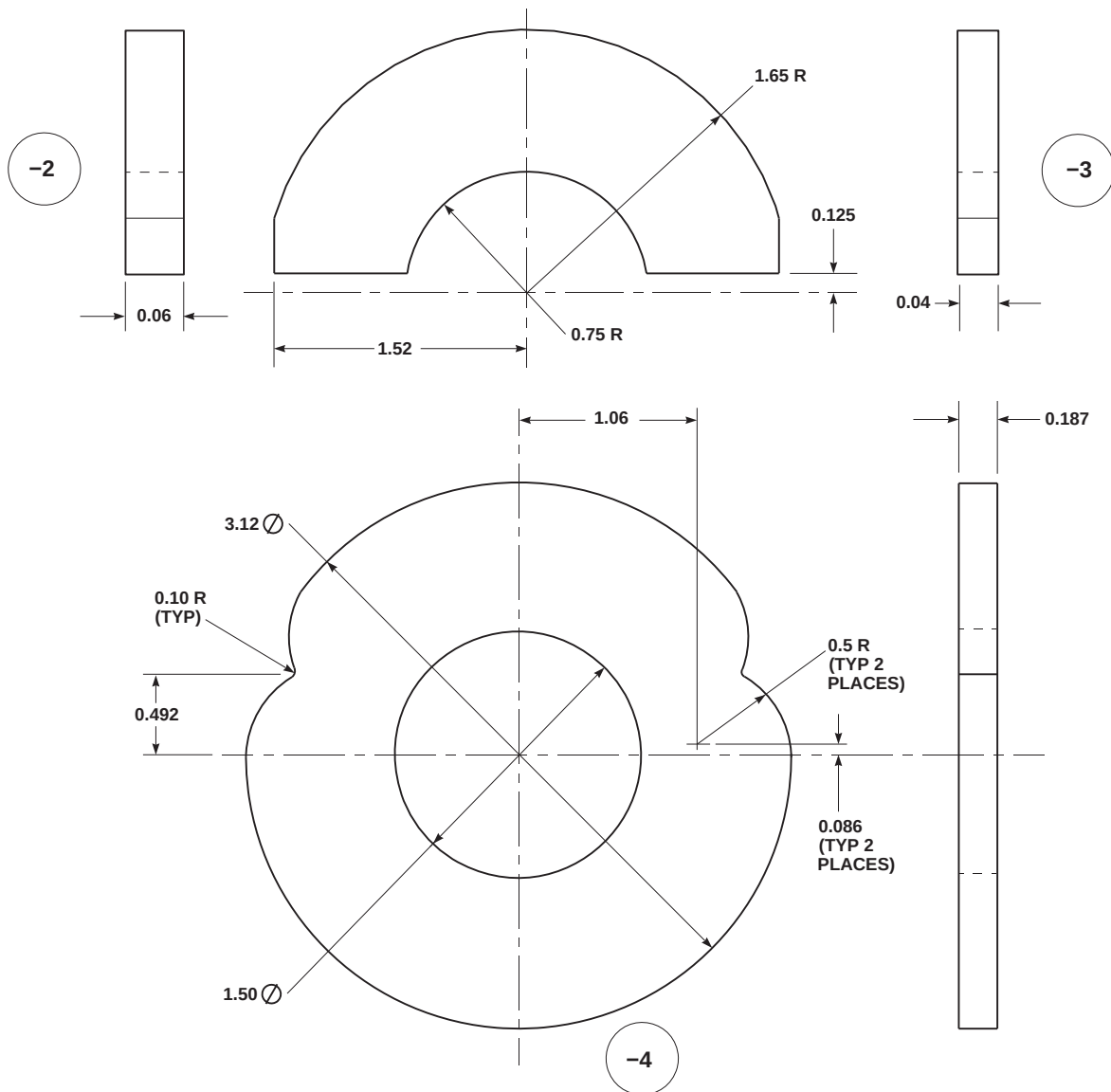
FIGURE H-213. BIFILAR BUSHINGS REPLACEMENT TOOLS (SHEET 2 OF 5)
