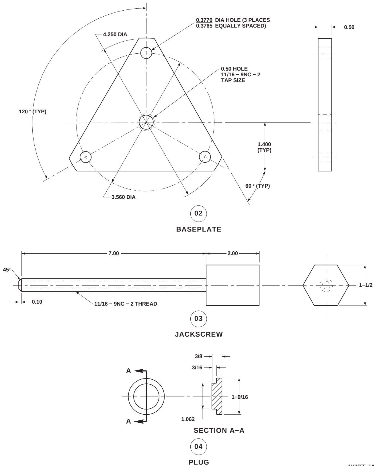
FIGURE H-50. FLANGE PULLER (SHEET 1 OF 2)
