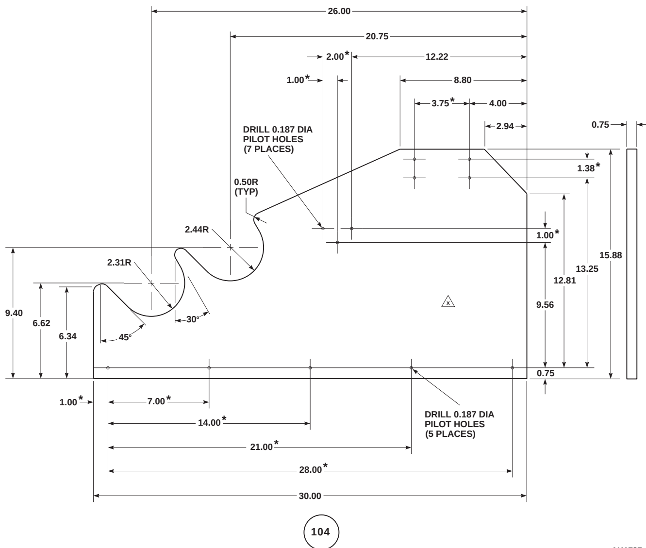
FIGURE H-110. PLYWOOD FRAME (SHEET 1 OF 2)
