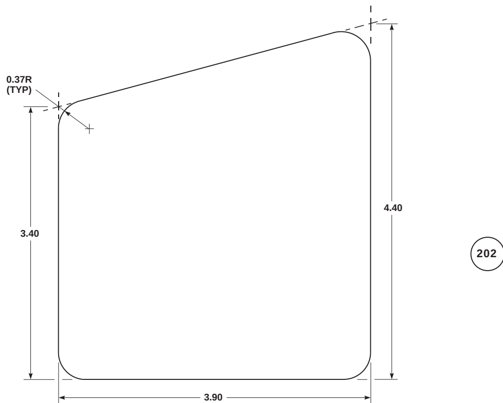
FIGURE H-131. FOIL PANEL UNUSUAL CONFIGURATION (SHEET 11 OF 43)
