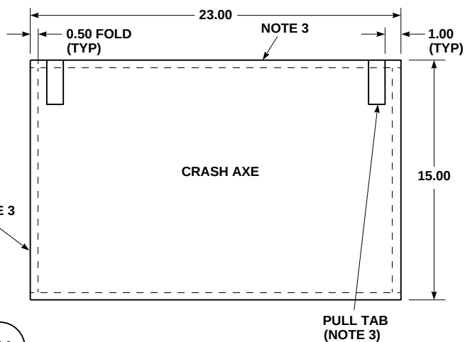
COVER FOLDED FOR SEWING
