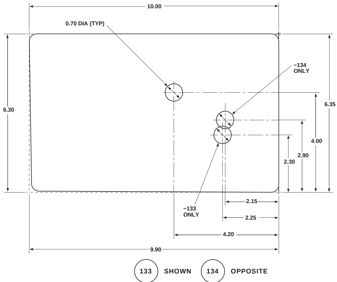
FIGURE H-131. FOIL PANEL UNUSUAL CONFIGURATION (SHEET 1 OF 43)
