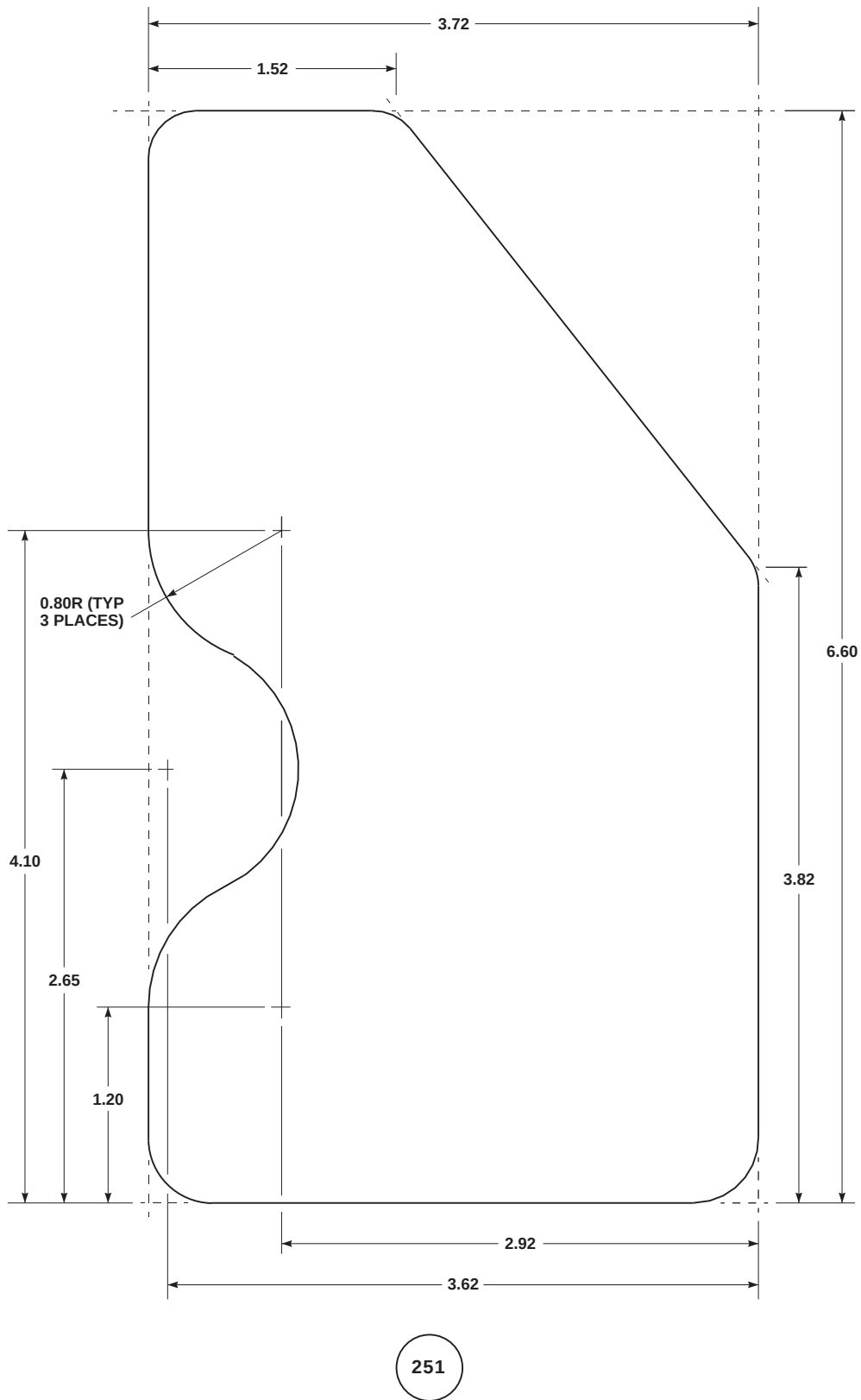
FIGURE H-131. FOIL PANEL UNUSUAL CONFIGURATION (SHEET 22 OF 43)
