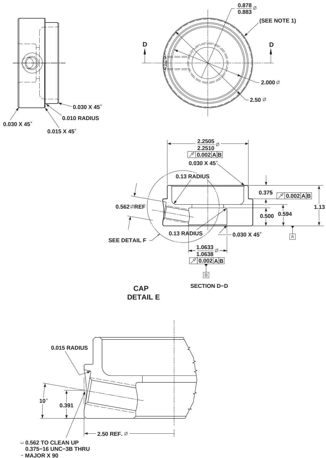
DETAIL F
