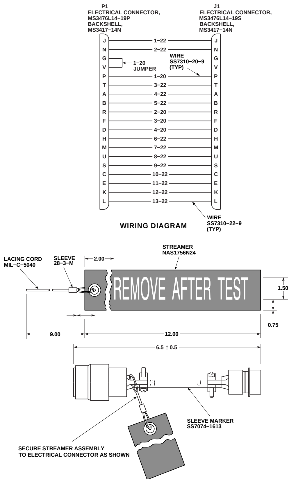
FIGURE H-175. DISPENSER TEST CABLE (SHEET 1 OF 2)
