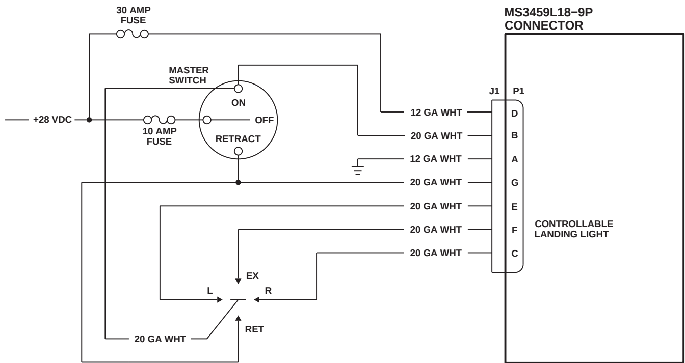
FIGURE H-249. SEARCHLIGHT TEST STAND (SHEET 3 OF 4)
