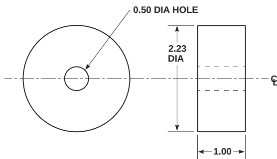
DETAIL A RUBBER DONUT (3 PLACES)
