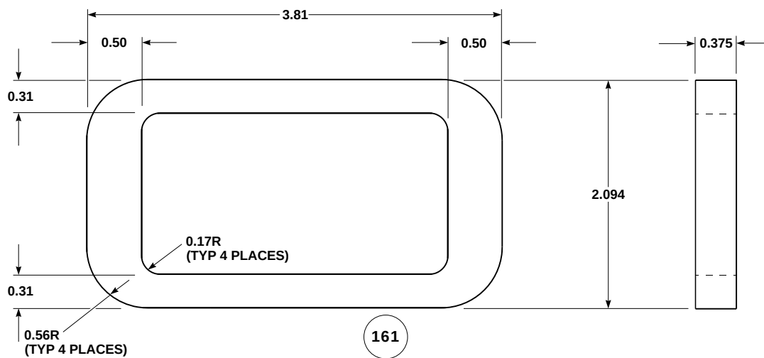
FIGURE H-42. DUCT INSTALLATION SEAL (SHEET 1 OF 2)
