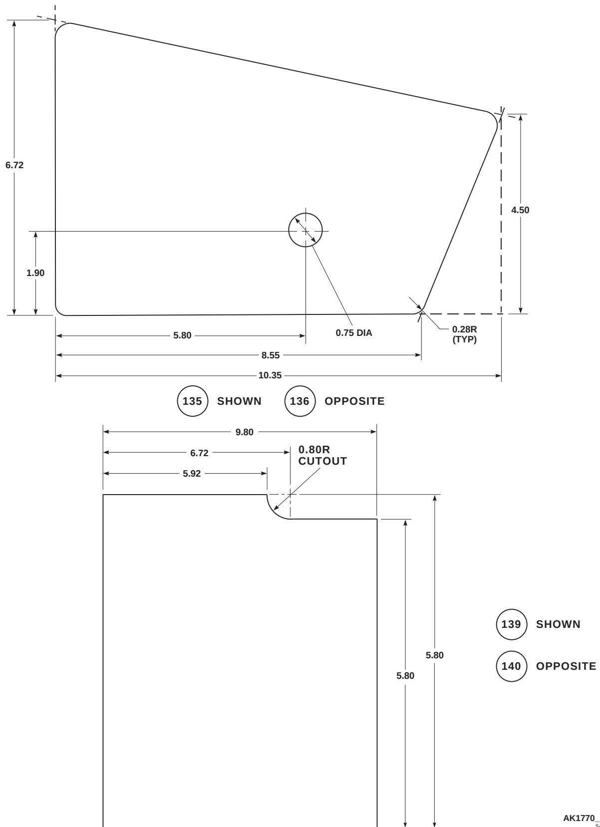
FIGURE H-131. FOIL PANEL UNUSUAL CONFIGURATION (SHEET 2 OF 43)
