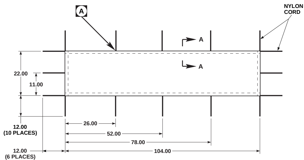
COVER FOLDED FOR SEWING
