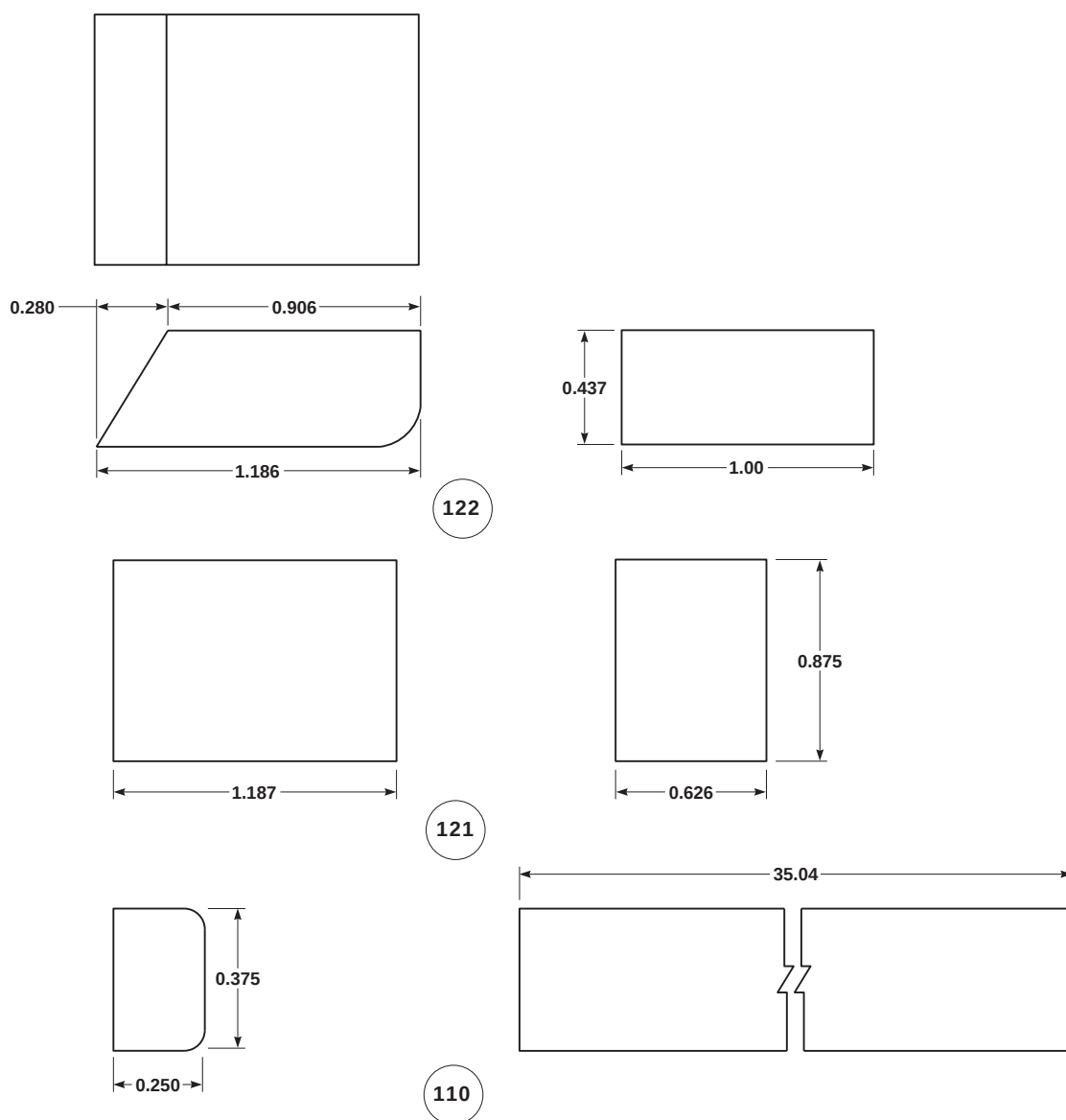
FIGURE H-240. CREW CHIEF'S WINDOW SEAL (SHEET 1 OF 2)
