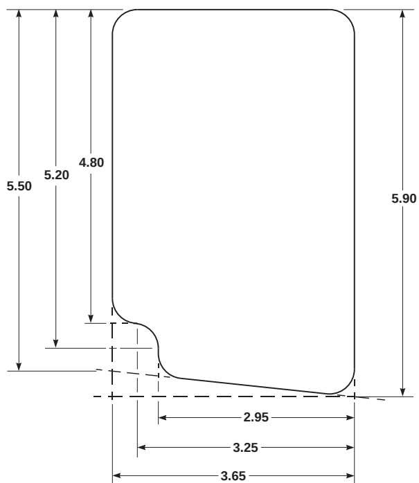
FIGURE H-131. FOIL PANEL UNUSUAL CONFIGURATION (SHEET 14 OF 43)
