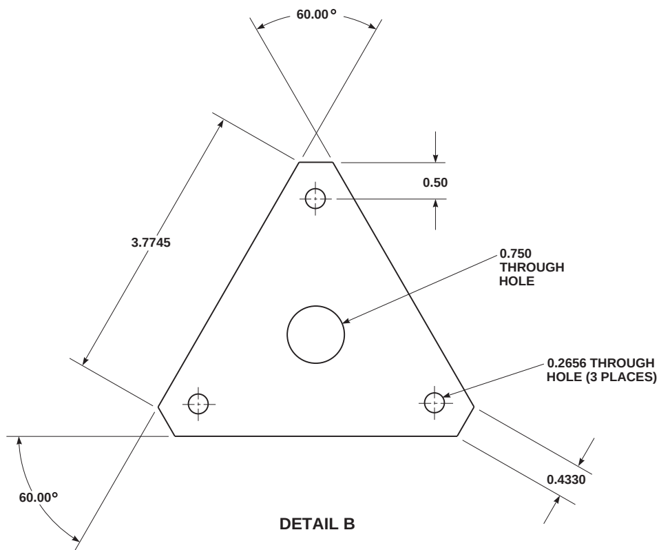
FIGURE H-262 OUTPUT DRIVE SHAFT PULLER (SHEET 2 OF 4)
