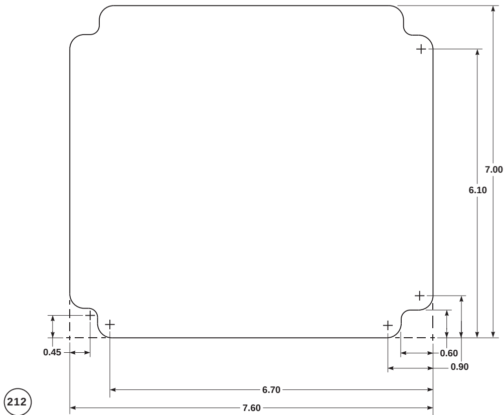
FIGURE H-131. FOIL PANEL UNUSUAL CONFIGURATION (SHEET 15 OF 43)
