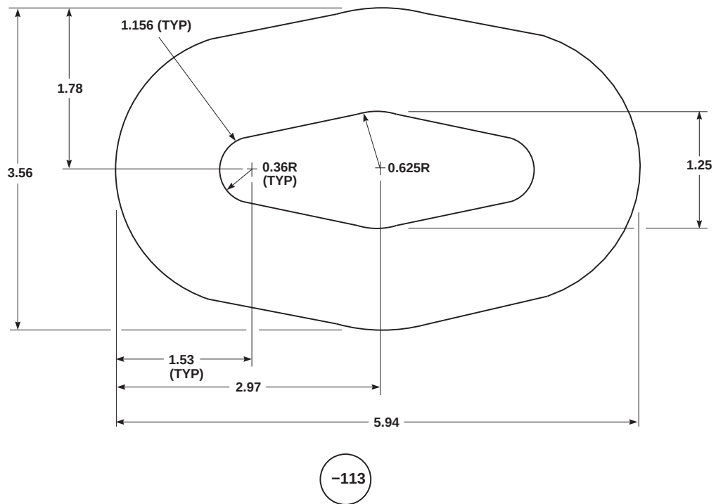
FIGURE H-54. TRANSMISSION DRIP PAN SEAL (SHEET 1 OF 2)
