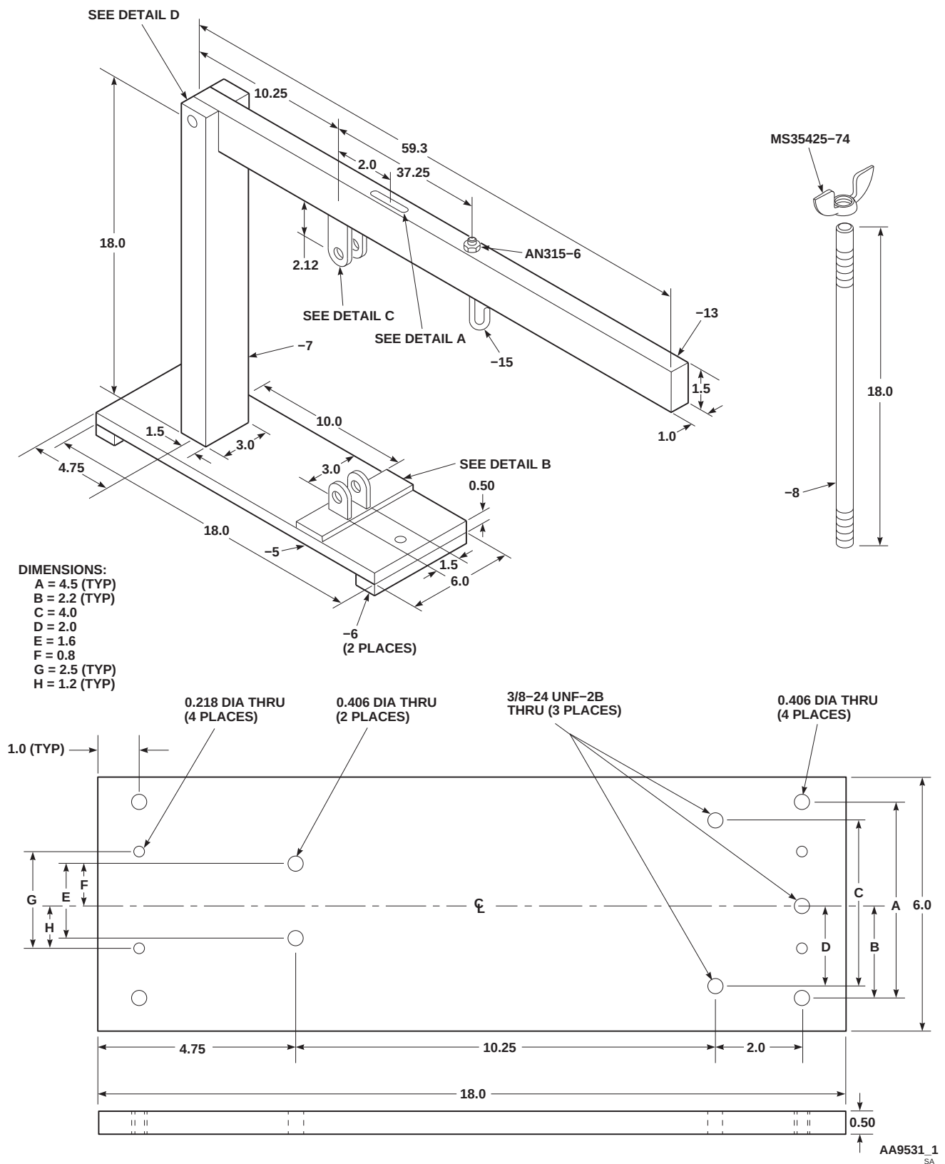
FIGURE H-227. MASTER BRAKE CYLINDER TEST STAND (SHEET 1 OF 4)
