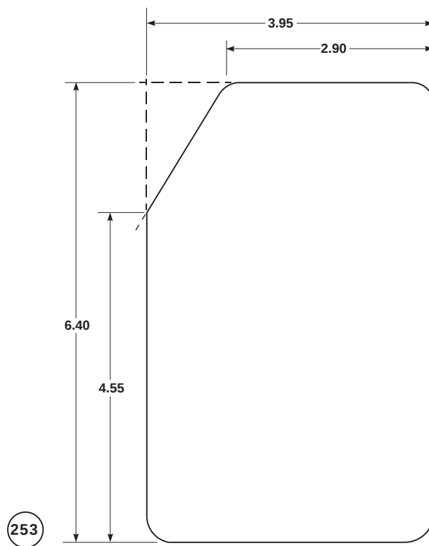
FIGURE H-131. FOIL PANEL UNUSUAL CONFIGURATION (SHEET 23 OF 43)
