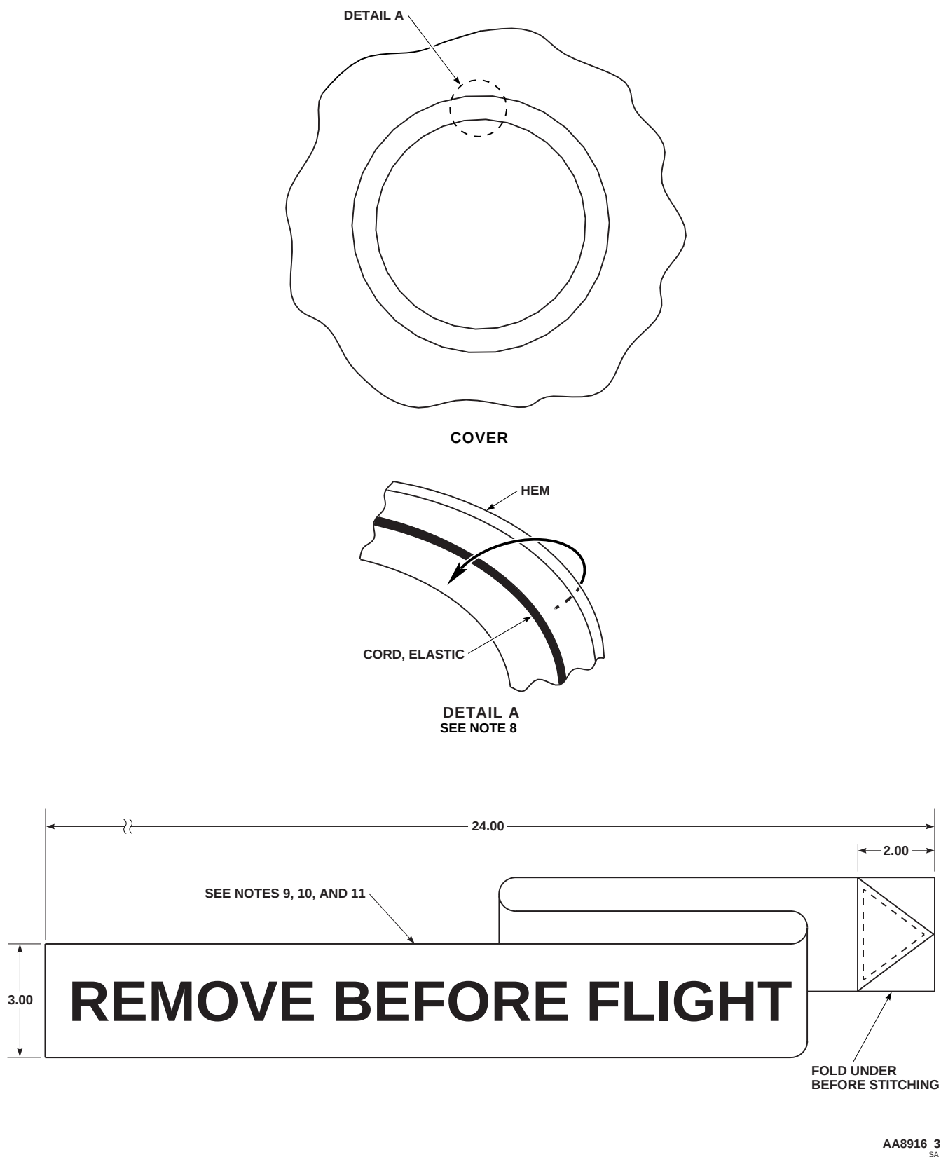
FIGURE H-214. CHAFF/FLARE DISPENSER COVER (SHEET 3 OF 4)
