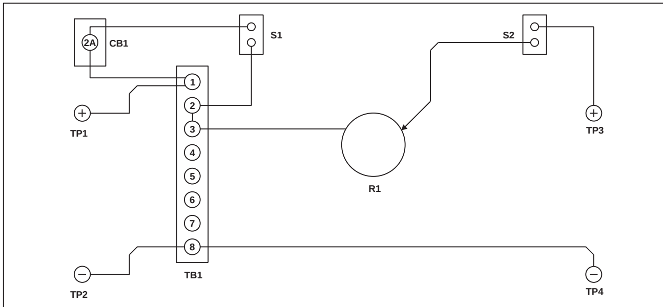
WIRING DIAGRAM
