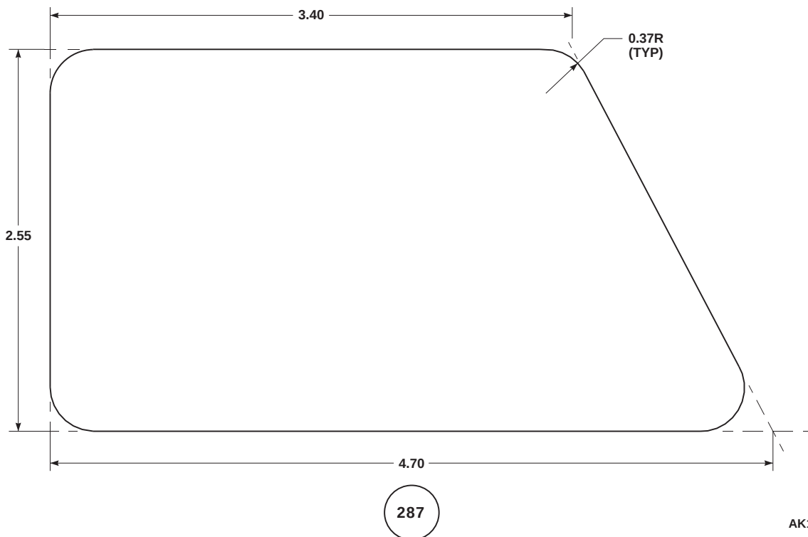
FIGURE H-131. FOIL PANEL UNUSUAL CONFIGURATION (SHEET 32 OF 43)
