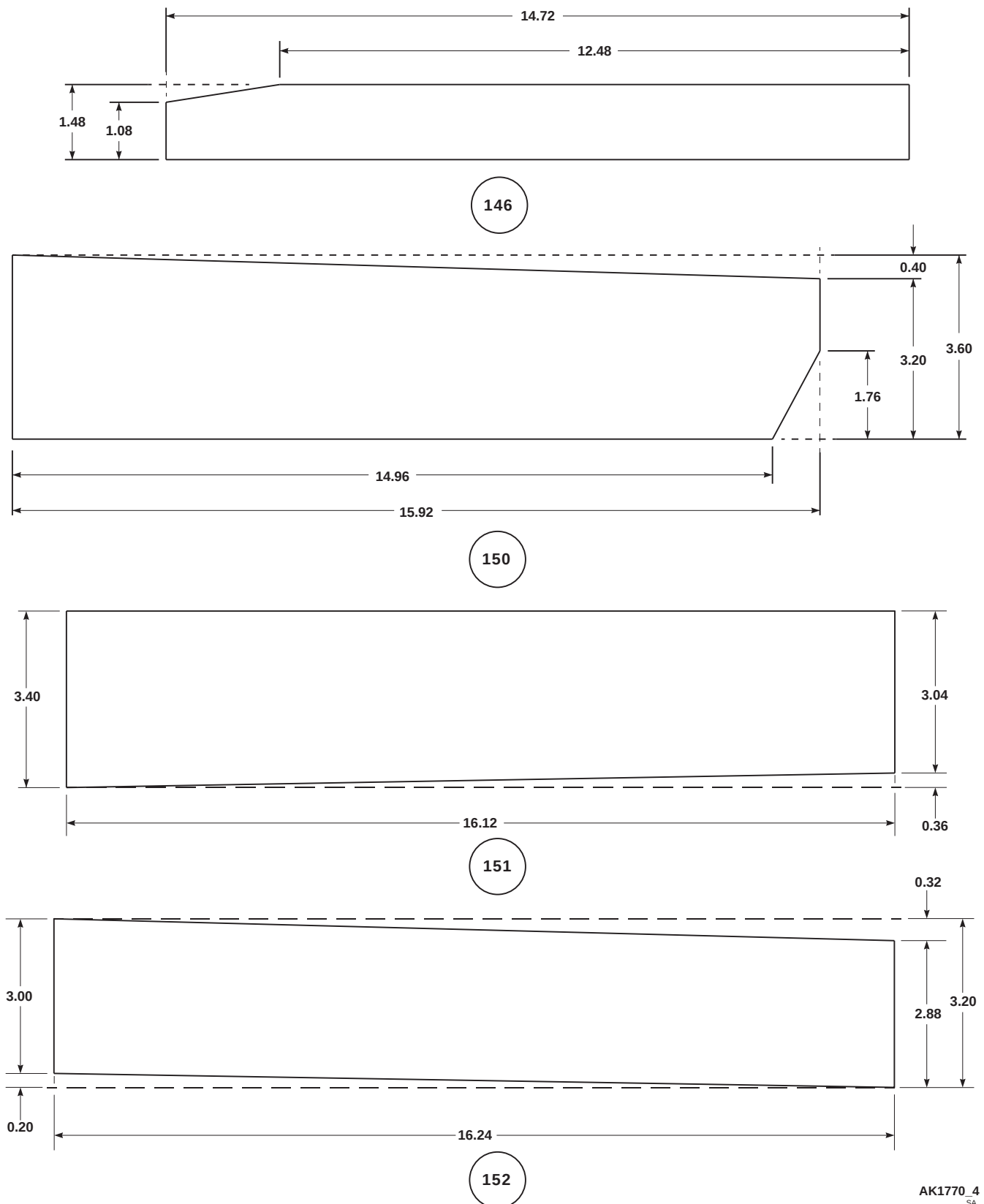
FIGURE H-131. FOIL PANEL UNUSUAL CONFIGURATION (SHEET 4 OF 43)
