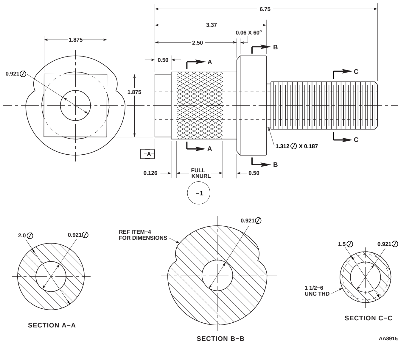
FIGURE H-213. BIFILAR BUSHINGS REPLACEMENT TOOLS (SHEET 1 OF 5)
