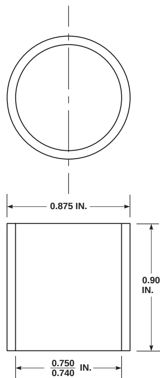
FIGURE H-221. TAIL LANDING GEAR LOCKPIN OVERSIZE BUSHING
