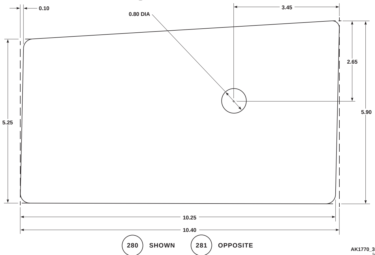
FIGURE H-131. FOIL PANEL UNUSUAL CONFIGURATION (SHEET 30 OF 43)
