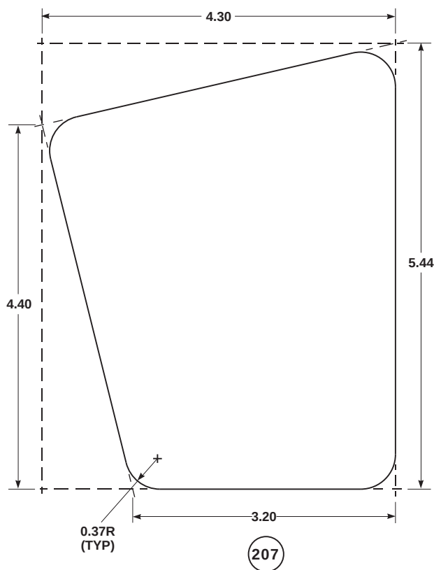
FIGURE H-131. FOIL PANEL UNUSUAL CONFIGURATION (SHEET 13 OF 43)
