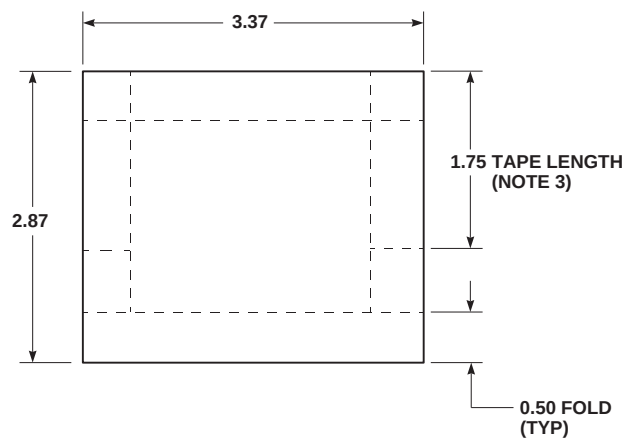
COVER FOLDED FOR SEWING
