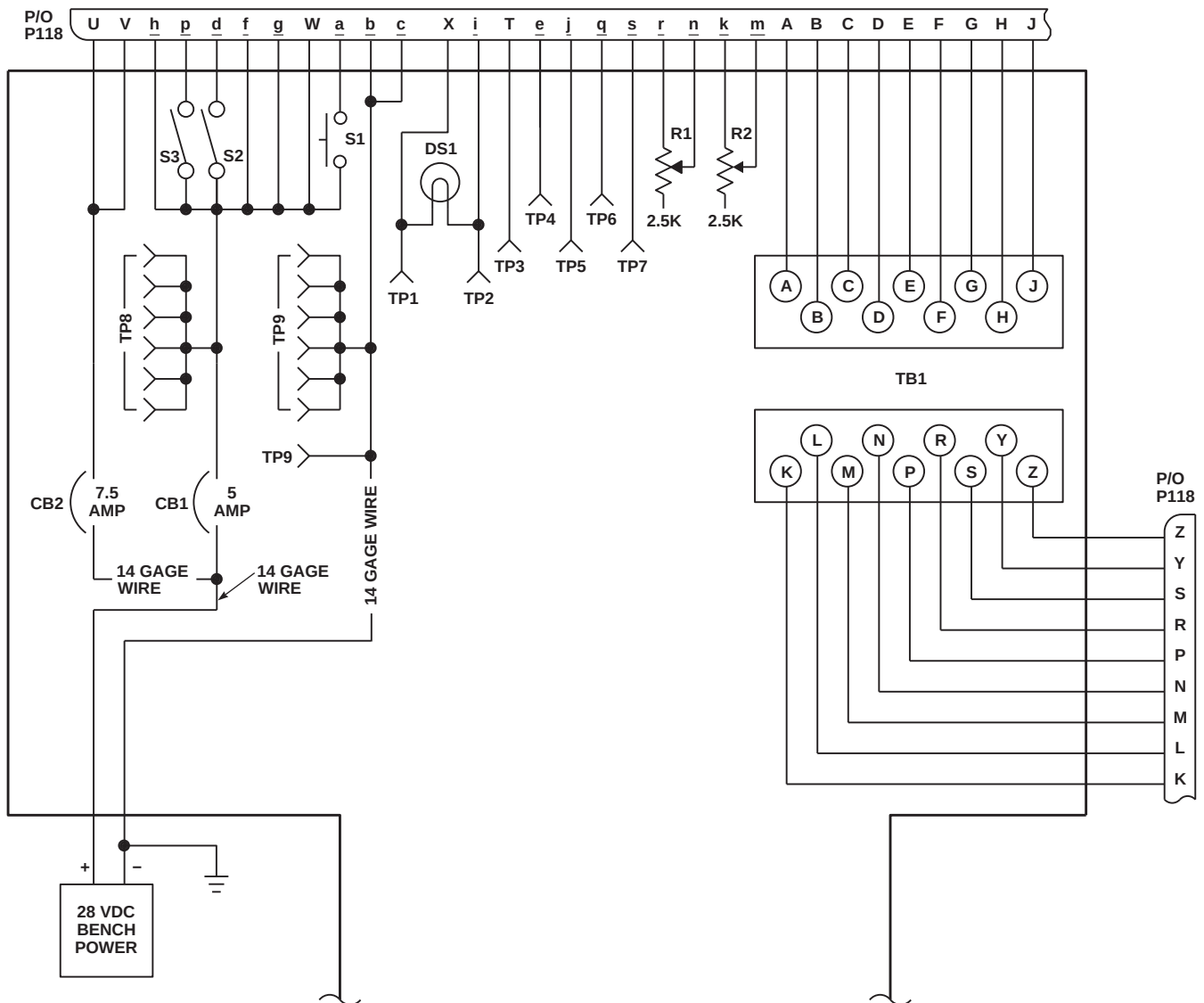
FIGURE H-53. CAUTION ADVISORY TEST ADAPTER (SHEET 1 OF 3)
