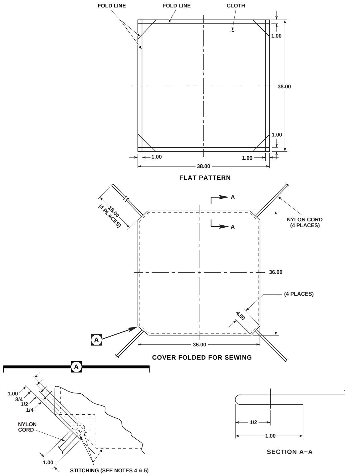
FIGURE H-190. TAIL ROTOR GEAR BOX COVER (SHEET 1 OF 2)
