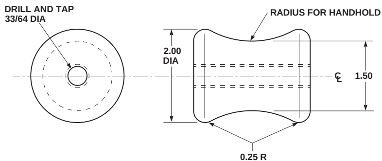
DETAIL D HAMMER
