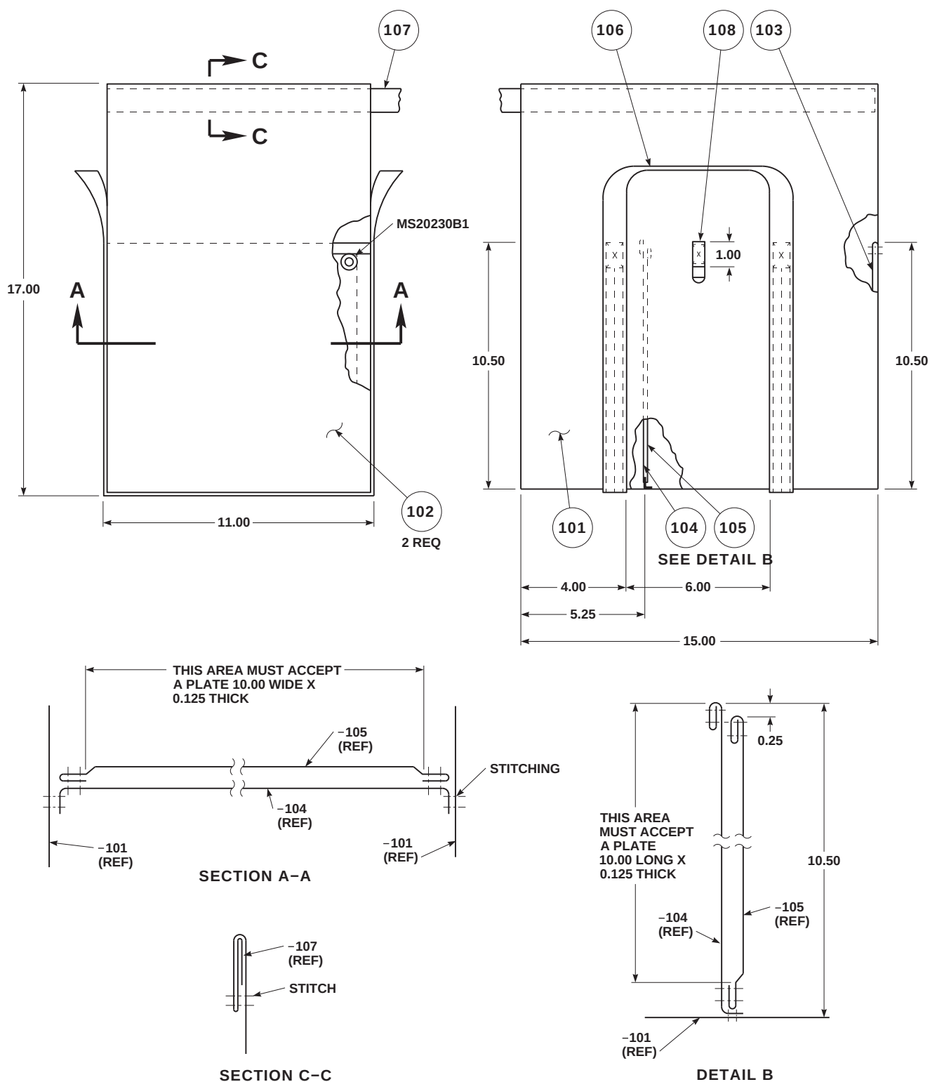
FIGURE H-120. STORAGE BAG (SHEET 1 OF 2)
