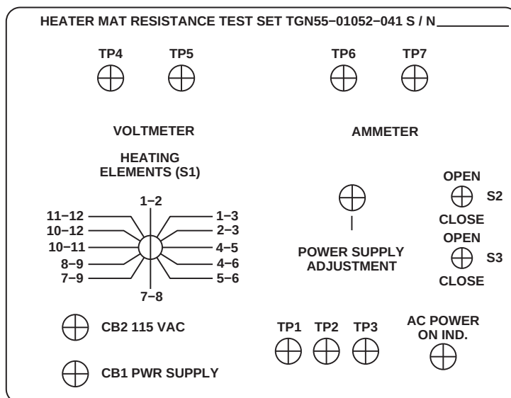
HEATER MAT RESISTANCE TEST SET FRONT PANEL MARKING
