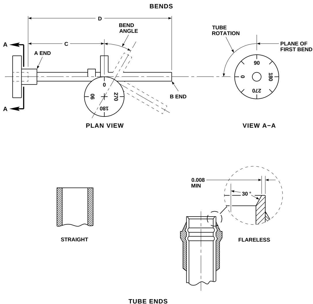
FIGURE H-41. HYDRAULIC TUBING (SHEET 1 OF 13)
