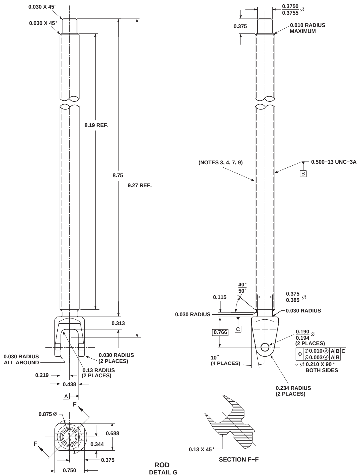
FIGURE H-266. MAIN ROTOR BLADE SOLID PIN REMOVAL TOOL (SHEET 5 OF 6)
