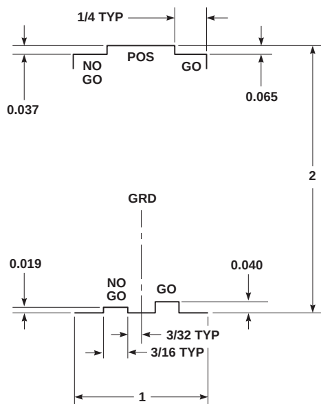
FIGURE H-135. BREECH CAP PLUG ASSEMBLY WRENCH AND GO/NO-GO BREECH CAP GAGE
