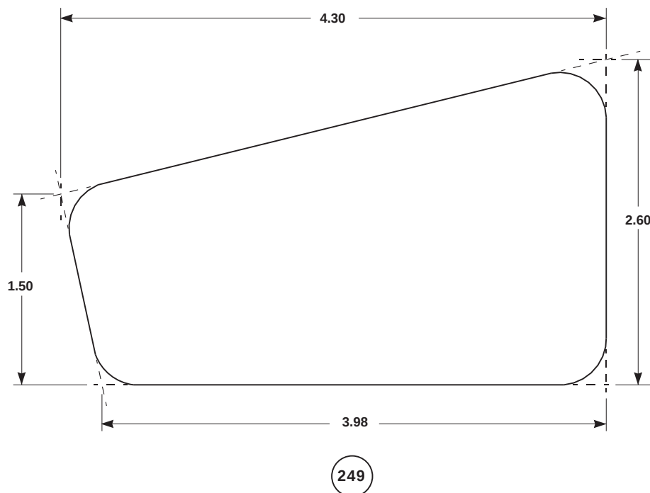
FIGURE H-131. FOIL PANEL UNUSUAL CONFIGURATION (SHEET 20 OF 43)
