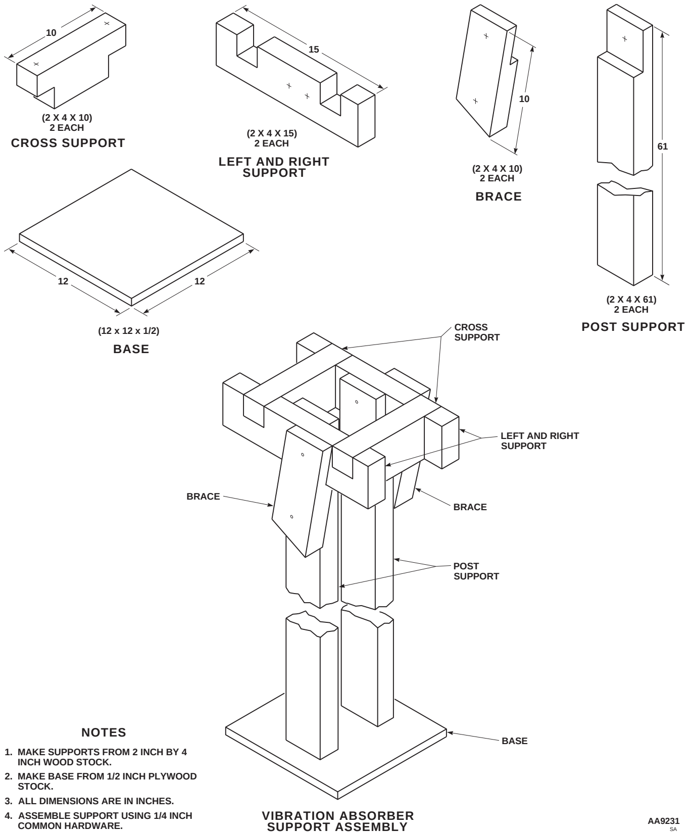
FIGURE H-220. VIBRATION ABSORBER SUPPORT ASSEMBLY
