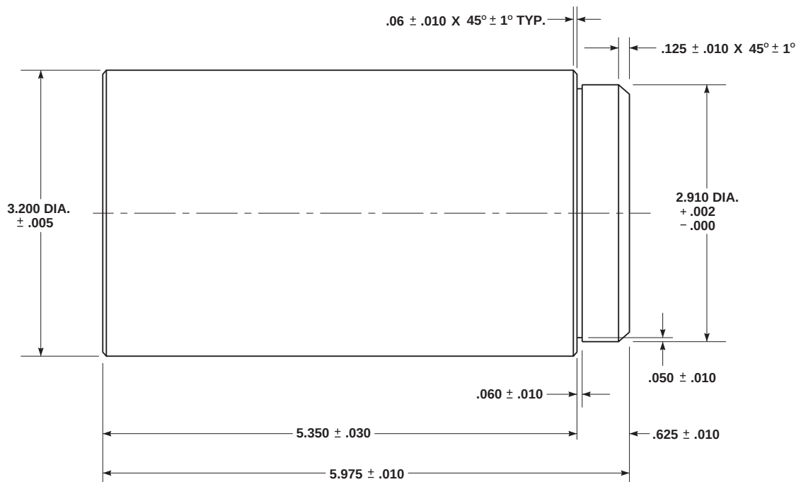
SPHERICAL BEARING SUPPORT (INSTALLATION) P/N 70102-08100-041T046.06
