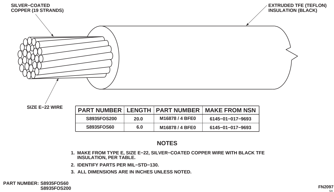
FIGURE H-17. HIGH-TEMPERATURE ELECTRICAL WIRE
