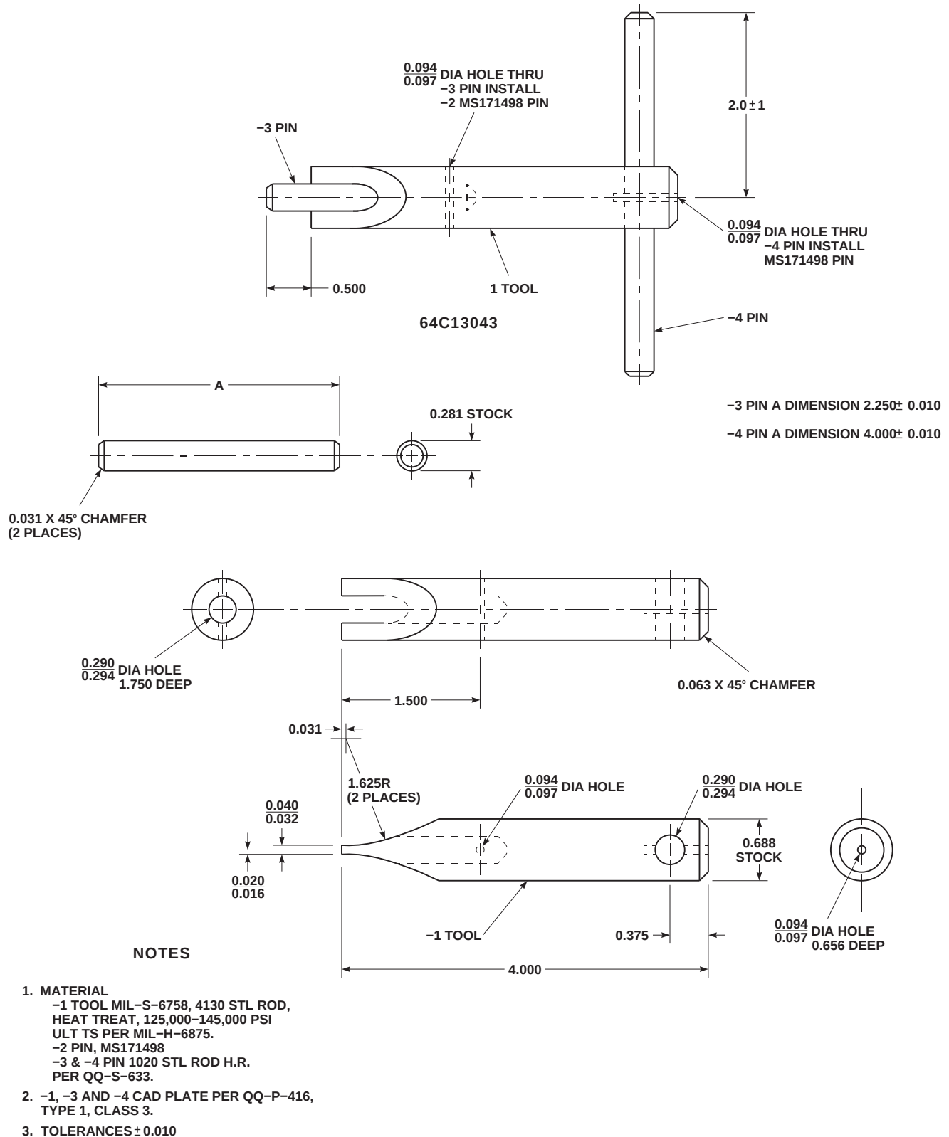
FIGURE H-136. PISTON GUIDE REMOVAL TOOL
