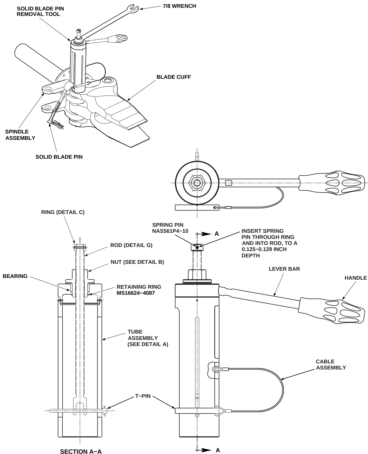
FIGURE H-266. MAIN ROTOR BLADE SOLID PIN REMOVAL TOOL (SHEET 1 OF 6)
