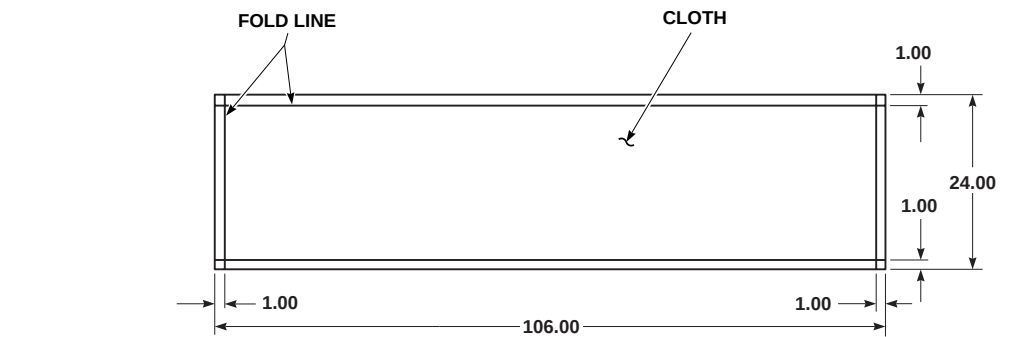
FLAT PATTERN
