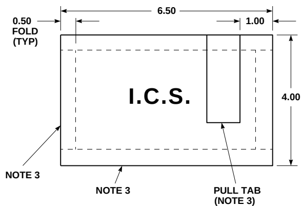
COVER FOLDED FOR SEWING
