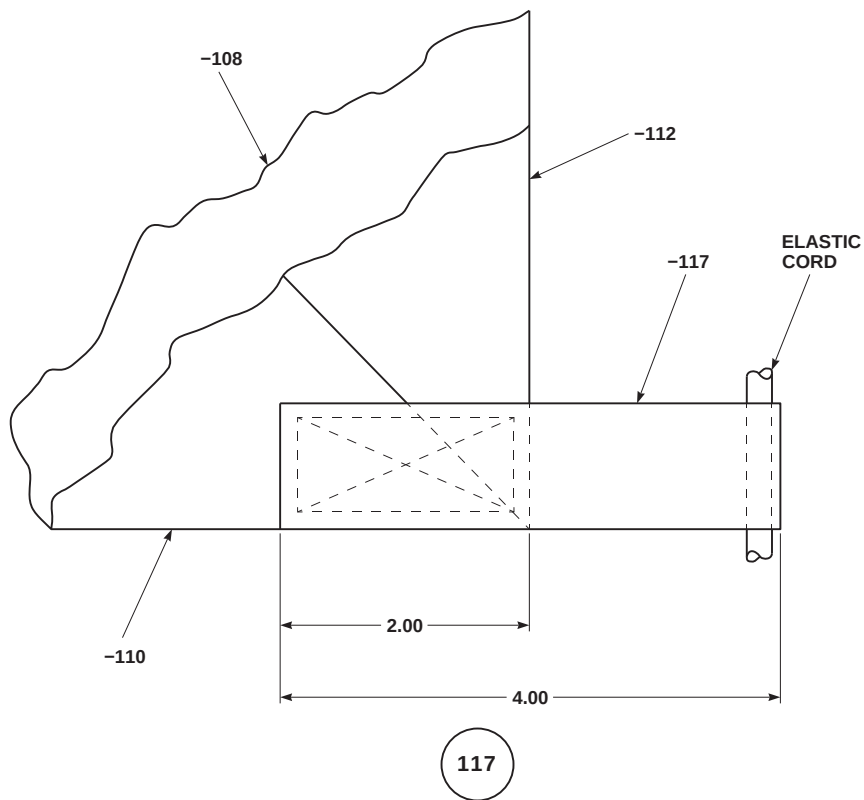
FIGURE H-33. OIL COOLER COVER ASSEMBLY (SHEET 6 OF 7)
