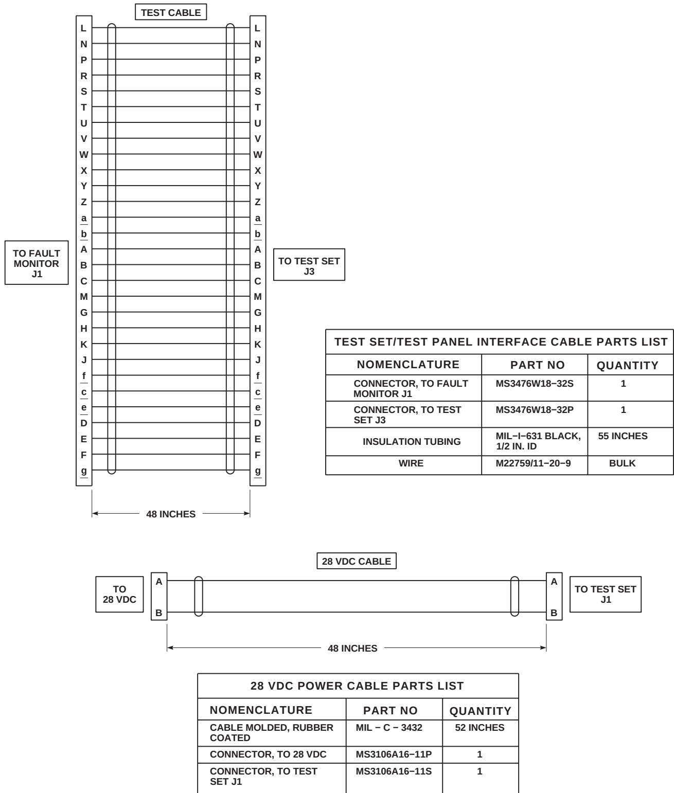
FIGURE H-155. BLADE DEICE TEST SET (SHEET 3 OF 4)
