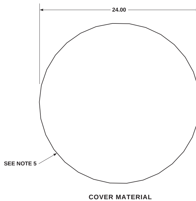
FIGURE H-214. CHAFF/FLARE DISPENSER COVER (SHEET 1 OF 4)
