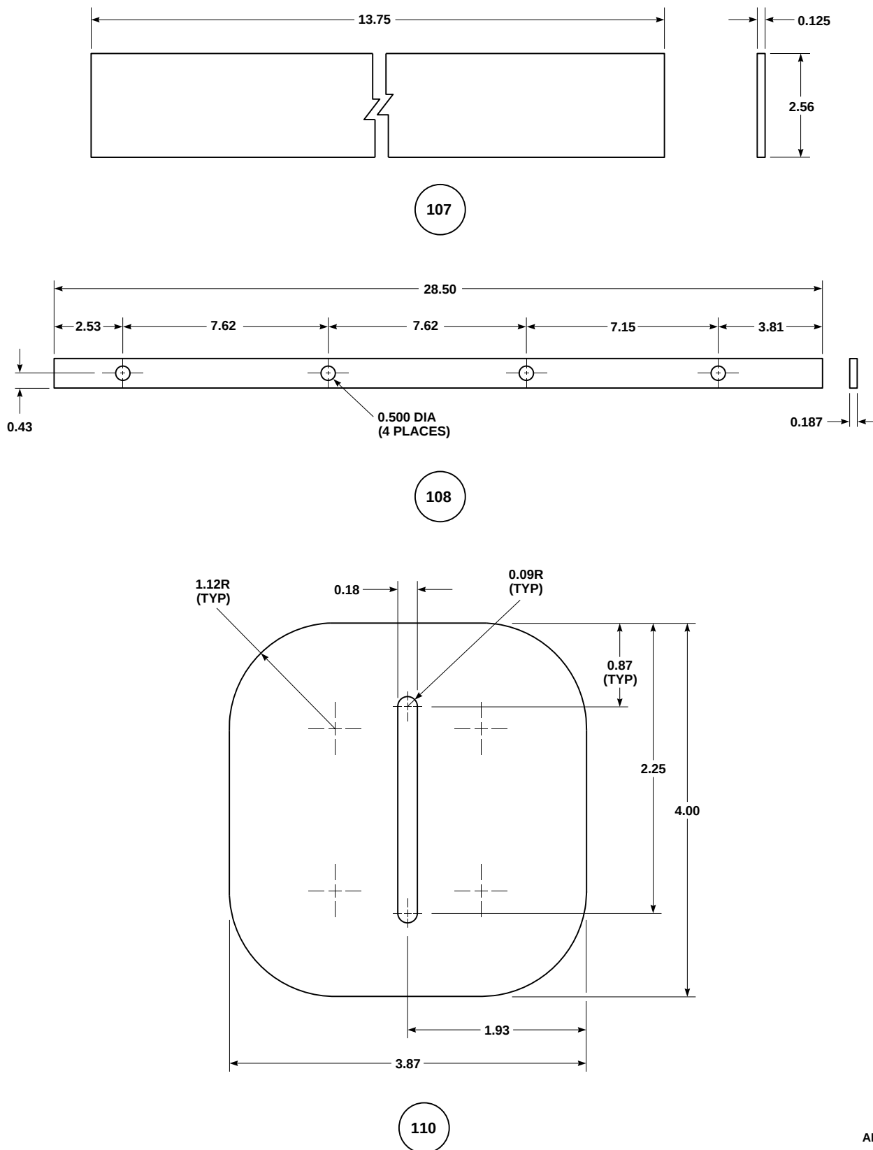
FIGURE H-77. CEILING PANEL SEAL (SHEET 1 OF 2)
