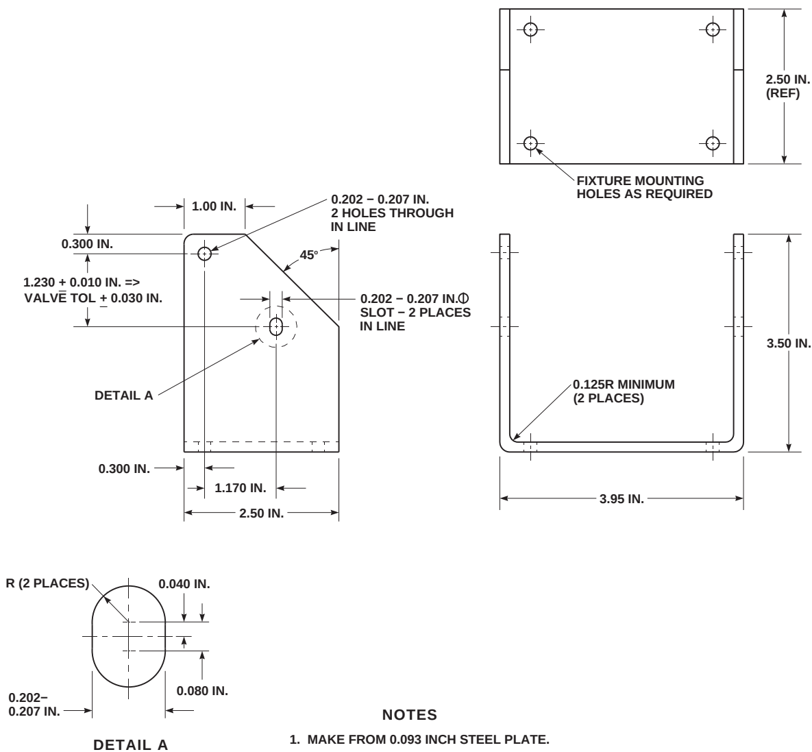
FIGURE H-202. VALVE TEST FIXTURE
