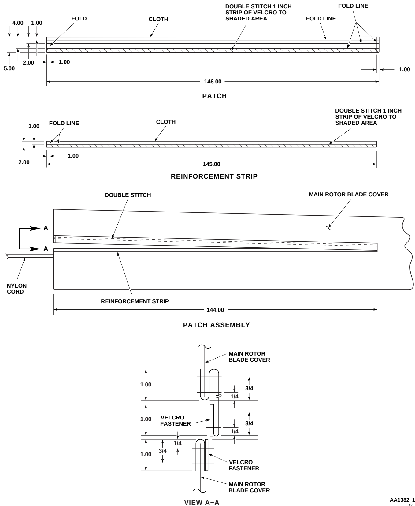
FIGURE H-191. PATCH ASSEMBLY (SHEET 1 OF 2)
