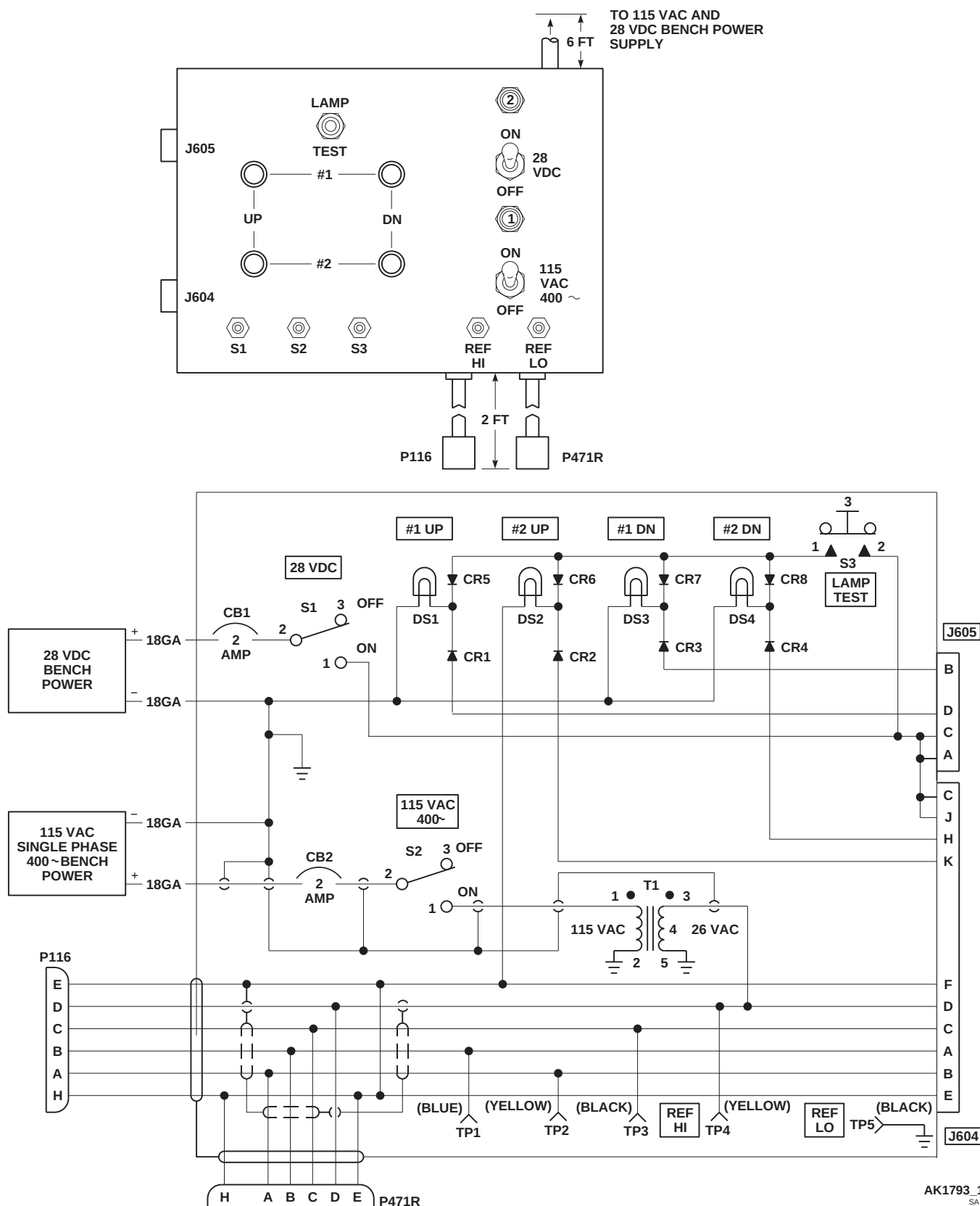
FIGURE H-154. STABILATOR POSITION SENSOR/LIMIT SWITCH TEST UNIT (SHEET 1 OF 3)
