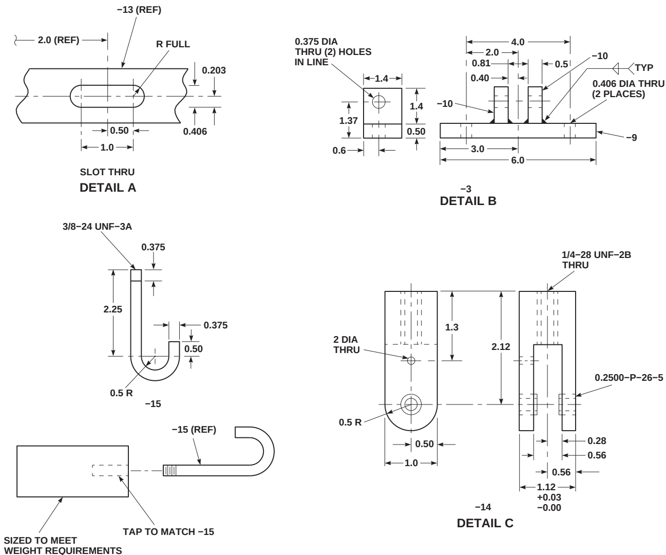
FIGURE H-227. MASTER BRAKE CYLINDER TEST STAND (SHEET 2 OF 4)
