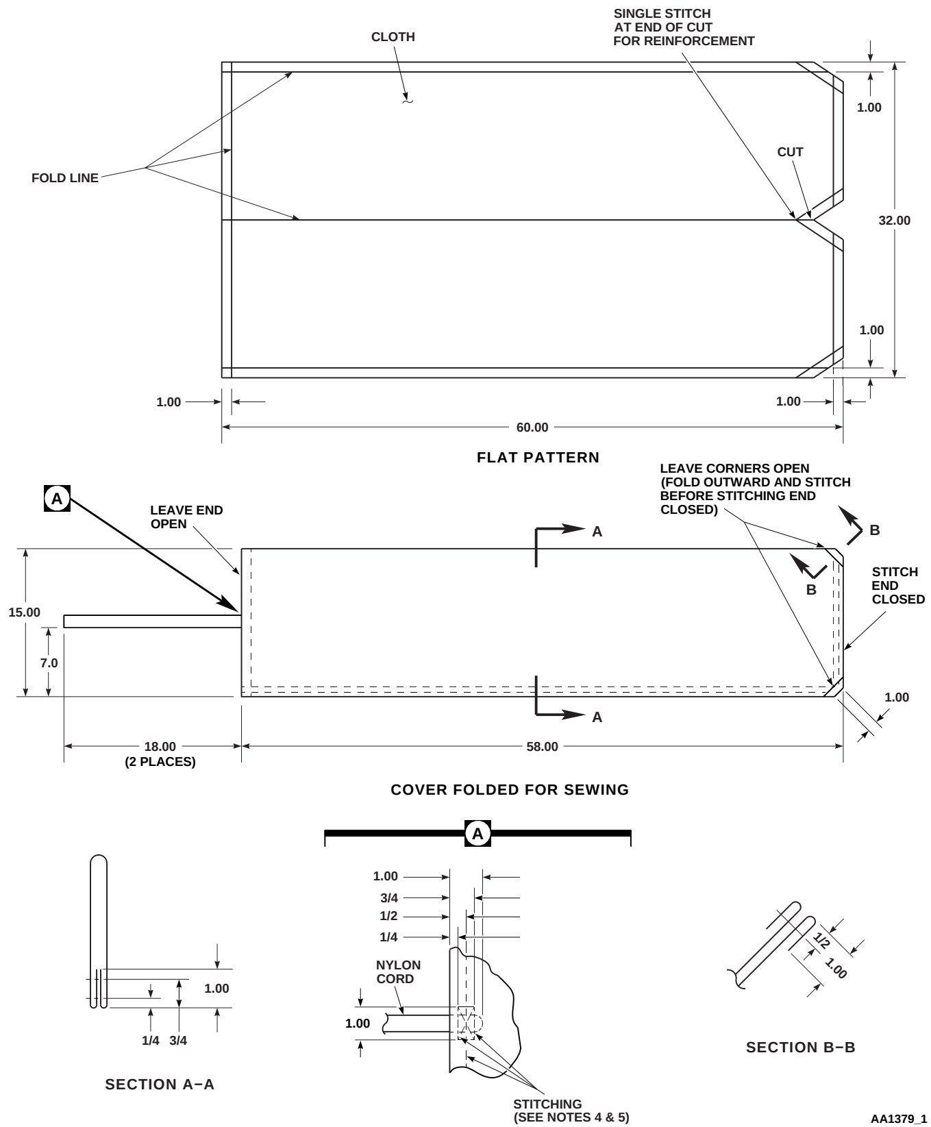
FIGURE H-188. TAIL ROTOR BLADE COVER (SHEET 1 OF 2)
