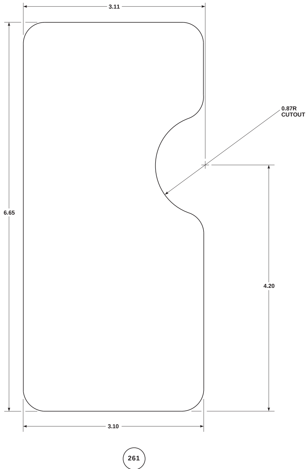
FIGURE H-131. FOIL PANEL UNUSUAL CONFIGURATION (SHEET 27 OF 43)
