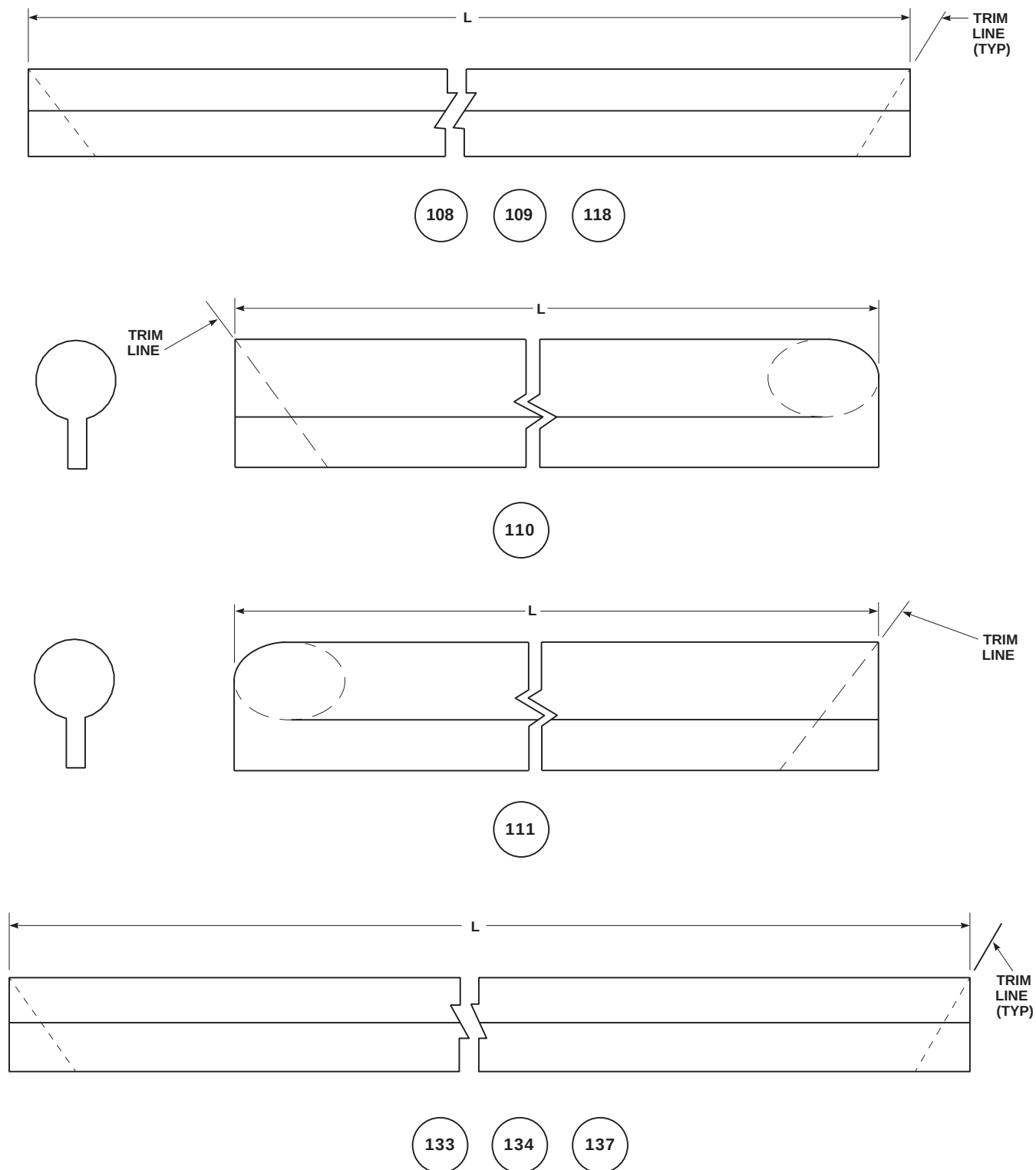
FIGURE H-65. ENGINE INLET FIREWALL SEAL (SHEET 1 OF 2)
