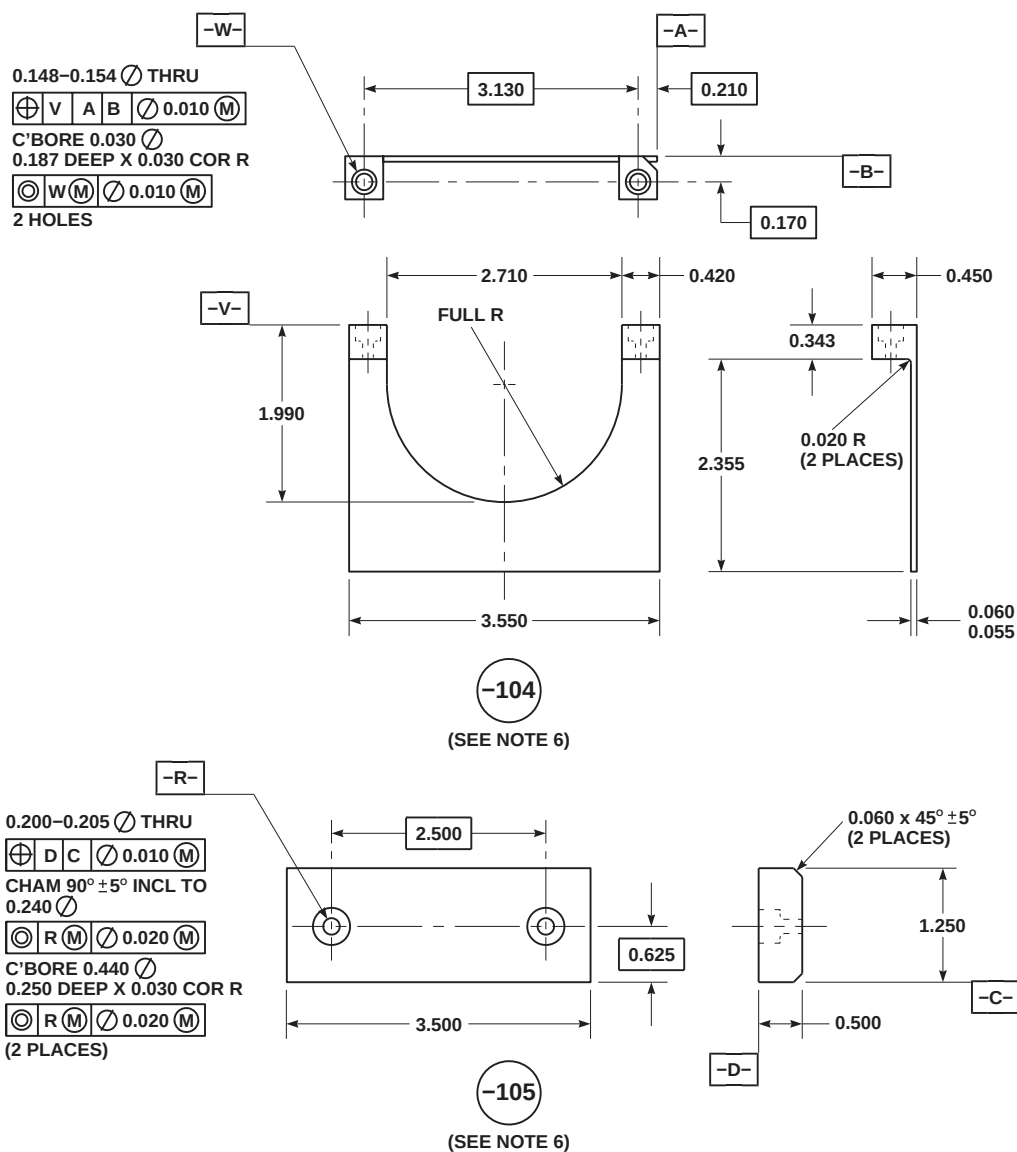
FIGURE H-223. MAIN ROTOR DAMPER HOLDING FIXTURE (SHEET 3 OF 4)
