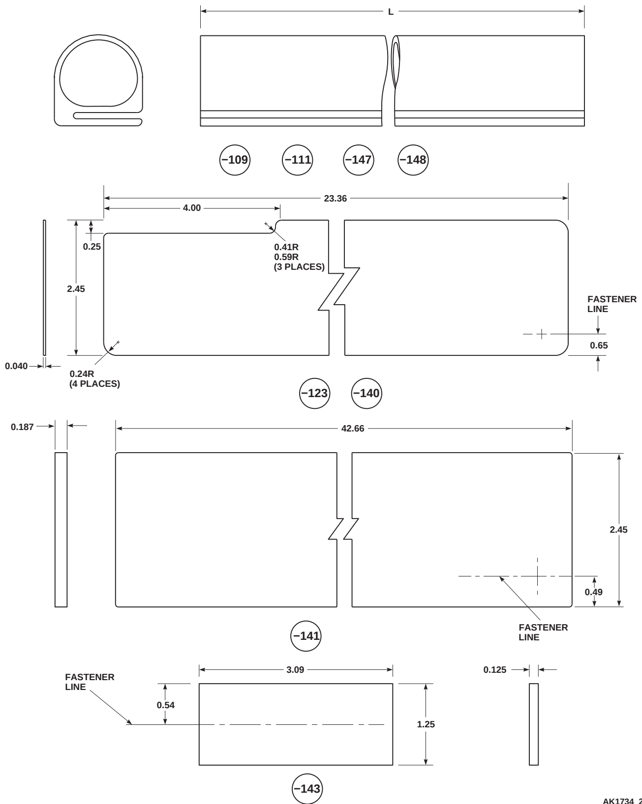
FIGURE H-76. CABIN DOOR SEAL (SHEET 2 OF 3)
