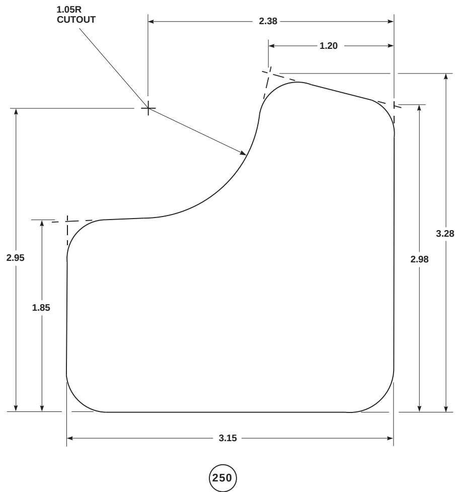
FIGURE H-131. FOIL PANEL UNUSUAL CONFIGURATION (SHEET 21 OF 43)
