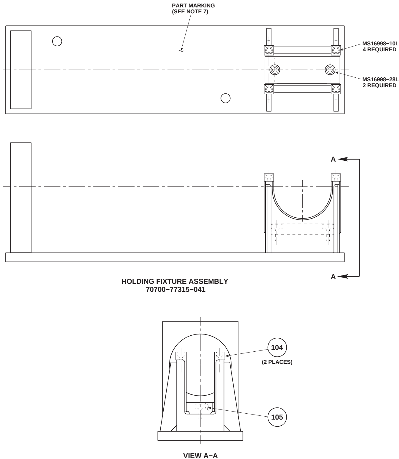
FIGURE H-223. MAIN ROTOR DAMPER HOLDING FIXTURE (SHEET 1 OF 4)
