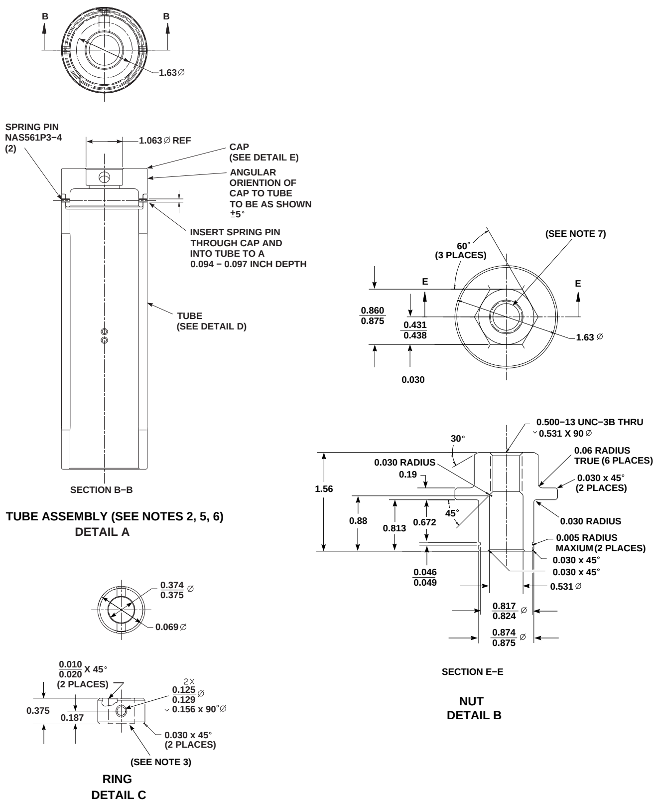
FIGURE H-266. MAIN ROTOR BLADE SOLID PIN REMOVAL TOOL (SHEET 2 OF 6)
