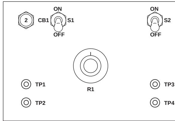
FRONT PANEL
