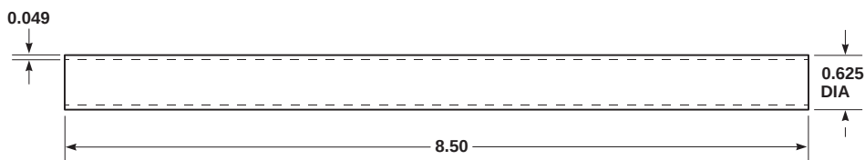
DETAIL B TUBING
